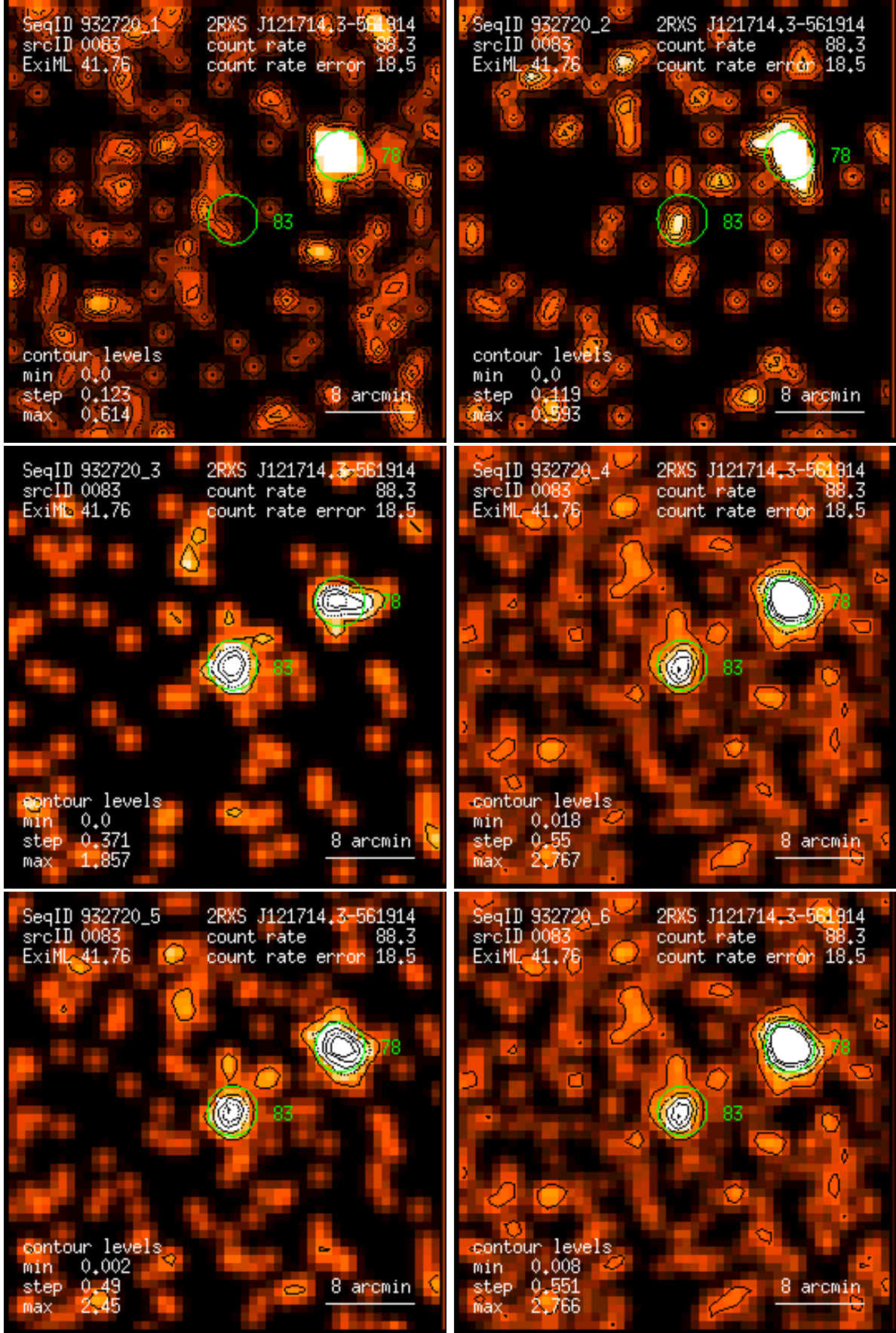
Figure 83: RASS 932720: detection 0083: band rate images, Gaussian filter: (1) PSPC channels 11 – 41, (2) 52 – 90, (3) 91 – 201, (4) 11 – 235, (5) 52 – 201, (6) 11 – 201. Broad band rates in counts/ks. Band rate contour levels in counts/ks/arcmin 2 .
