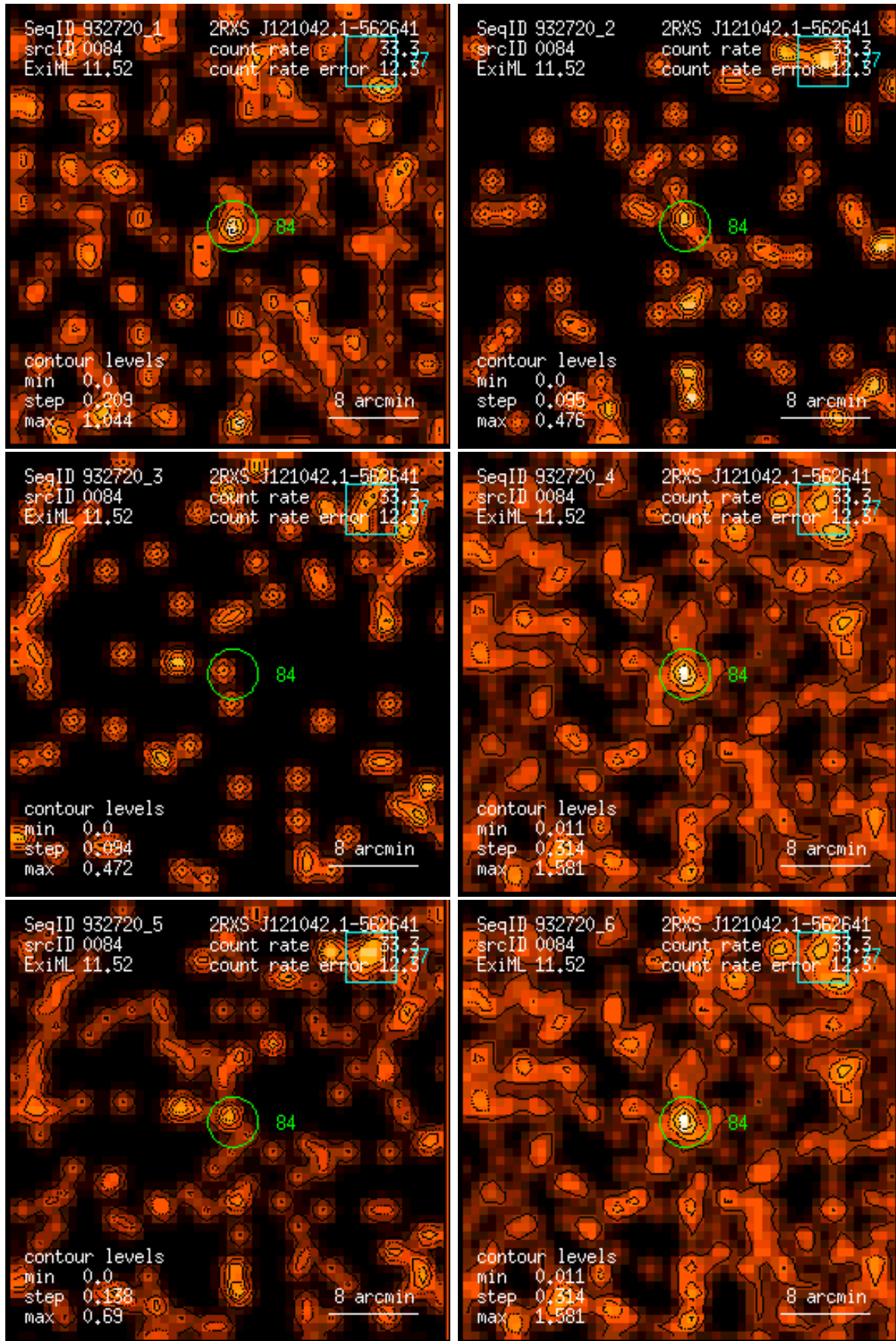
Figure 84: RASS 932720: detection 0084: band rate images, Gaussian filter: (1) PSPC channels 11 – 41, (2) 52 – 90, (3) 91 – 201, (4) 11 – 235, (5) 52 – 201, (6) 11 – 201. Broad band rates in counts/ks. Band rate contour levels in counts/ks/arcmin 2 .
