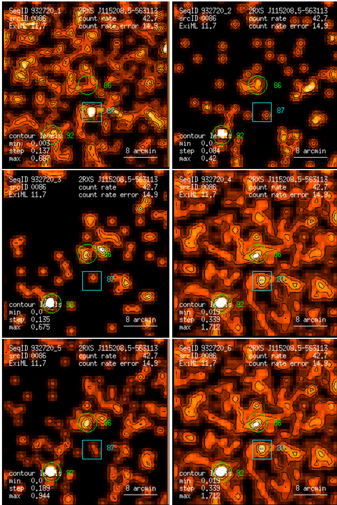
Figure 86: RASS 932720: detection 0086: band rate images, Gaussian filter: (1) PSPC channels 11 – 41, (2) 52 – 90, (3) 91 – 201, (4) 11 – 235, (5) 52 – 201, (6) 11 – 201. Broad band rates in counts/ks. Band rate contour levels in counts/ks/arcmin 2 .
