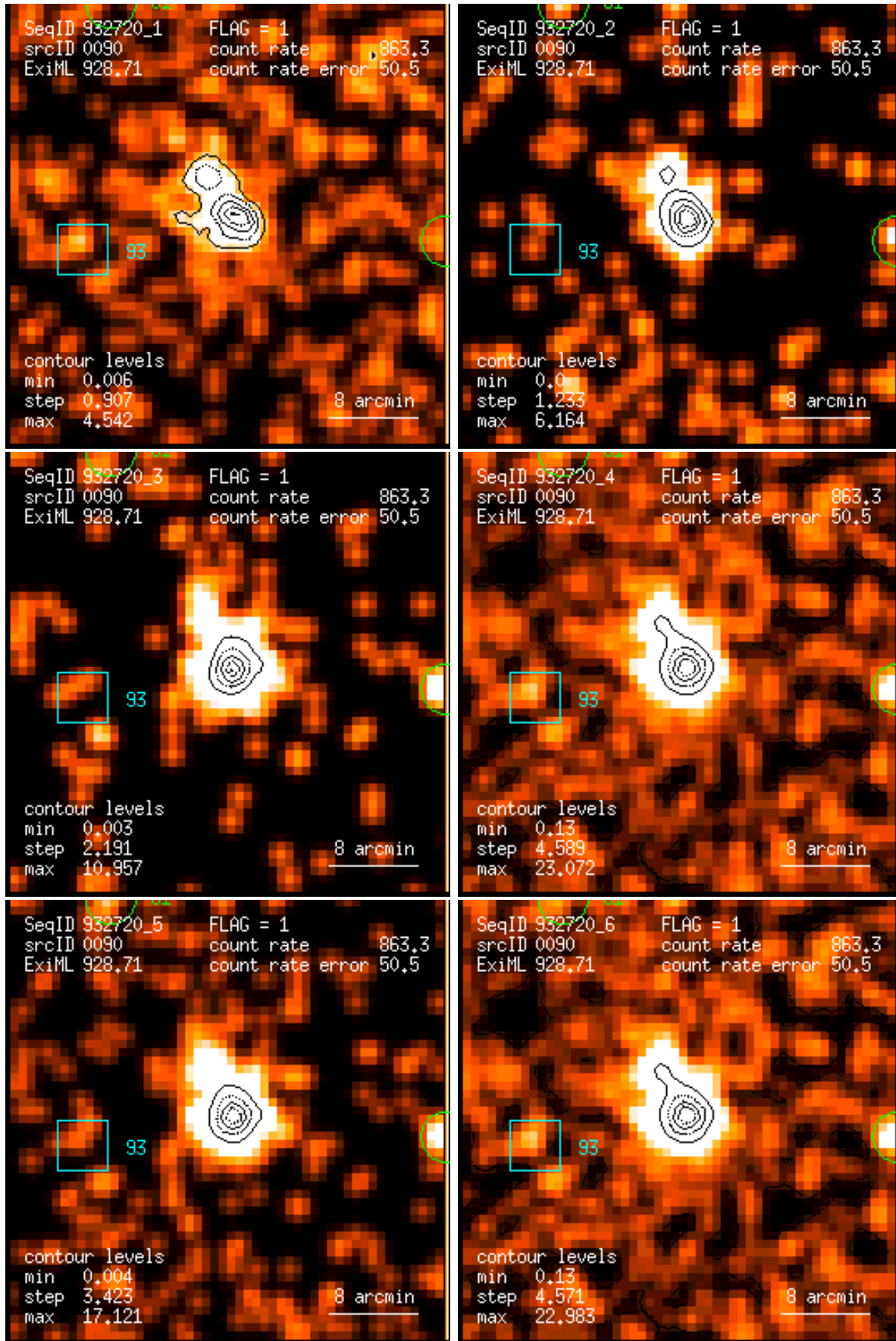
Figure 90: RASS 932720: detection 0090: band rate images, Gaussian filter: (1) PSPC channels 11 – 41, (2) 52 – 90, (3) 91 – 201, (4) 11 – 235, (5) 52 – 201, (6) 11 – 201. Broad band rates in counts/ks. Band rate contour levels in counts/ks/arcmin 2 .
