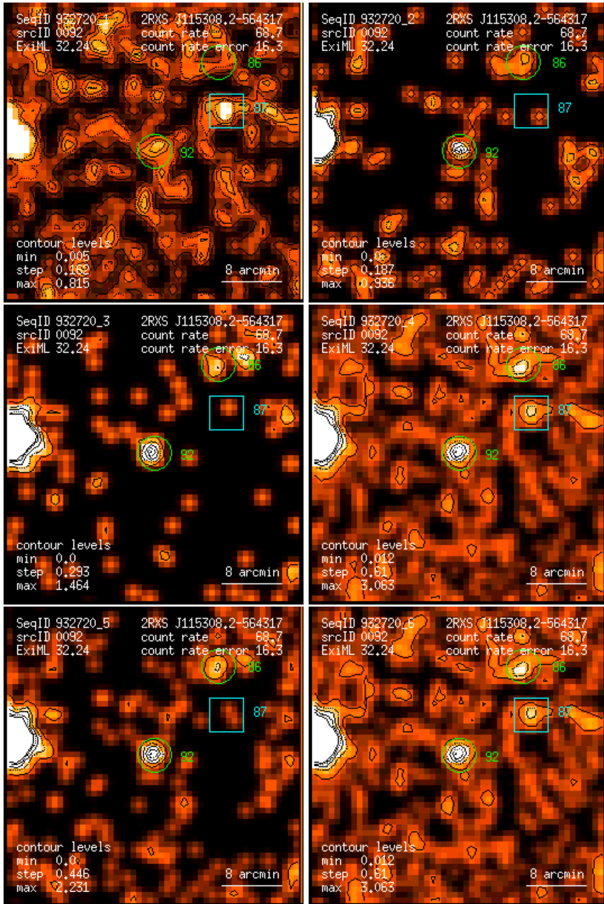
Figure 92: RASS 932720: detection 0092: band rate images, Gaussian filter: (1) PSPC channels 11 – 41, (2) 52 – 90, (3) 91 – 201, (4) 11 – 235, (5) 52 – 201, (6) 11 – 201. Broad band rates in counts/ks. Band rate contour levels in counts/ks/arcmin 2 .
