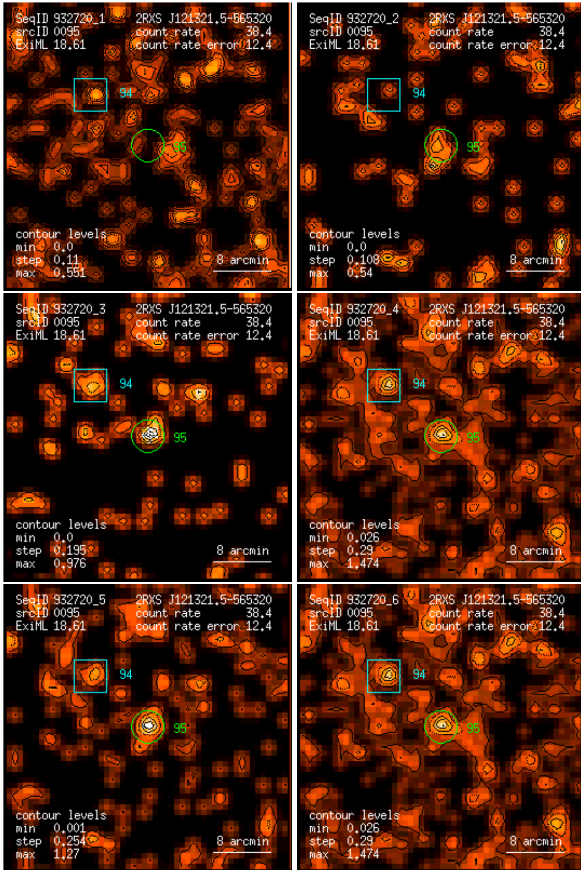
Figure 95: RASS 932720: detection 0095: band rate images, Gaussian filter: (1) PSPC channels 11 – 41, (2) 52 – 90, (3) 91 – 201, (4) 11 – 235, (5) 52 – 201, (6) 11 – 201. Broad band rates in counts/ks. Band rate contour levels in counts/ks/arcmin 2 .
