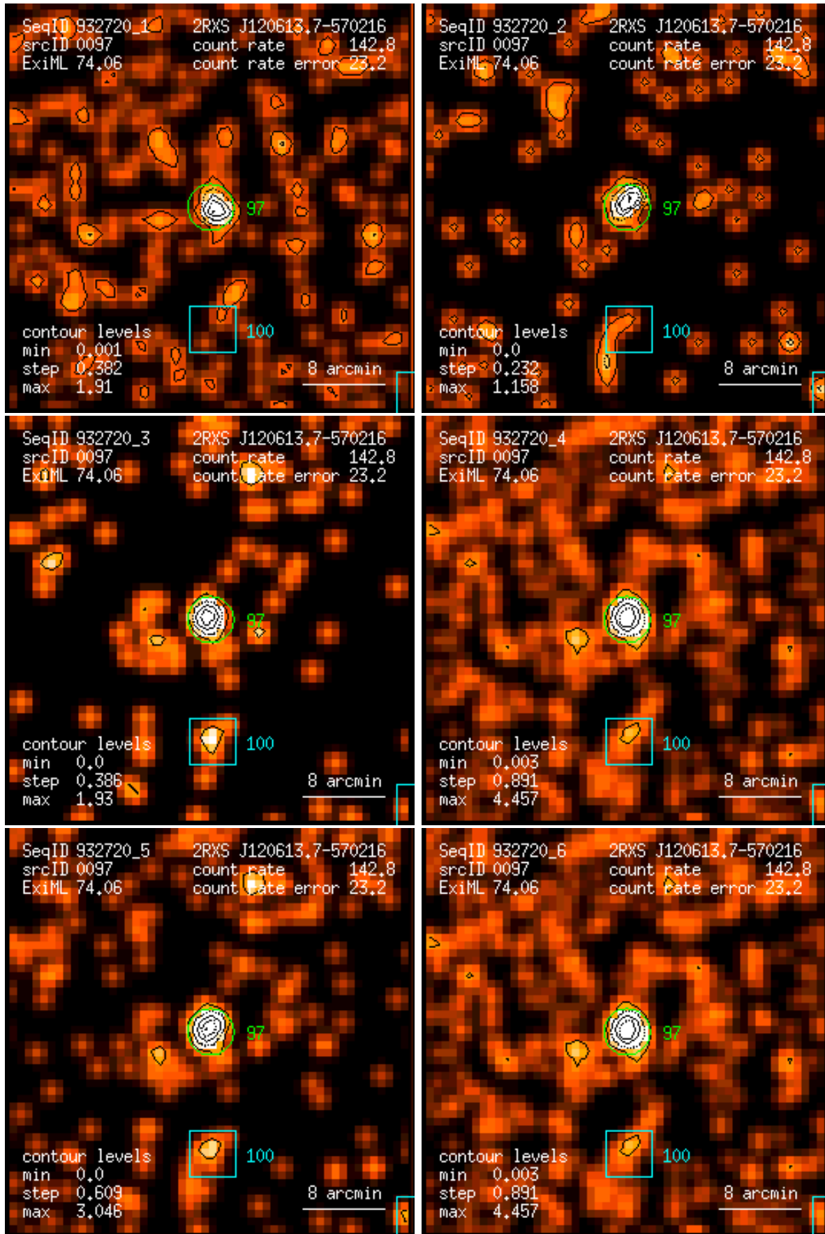
Figure 97: RASS 932720: detection 0097: band rate images, Gaussian filter: (1) PSPC channels 11 – 41, (2) 52 – 90, (3) 91 – 201, (4) 11 – 235, (5) 52 – 201, (6) 11 – 201. Broad band rates in counts/ks. Band rate contour levels in counts/ks/arcmin 2 .
