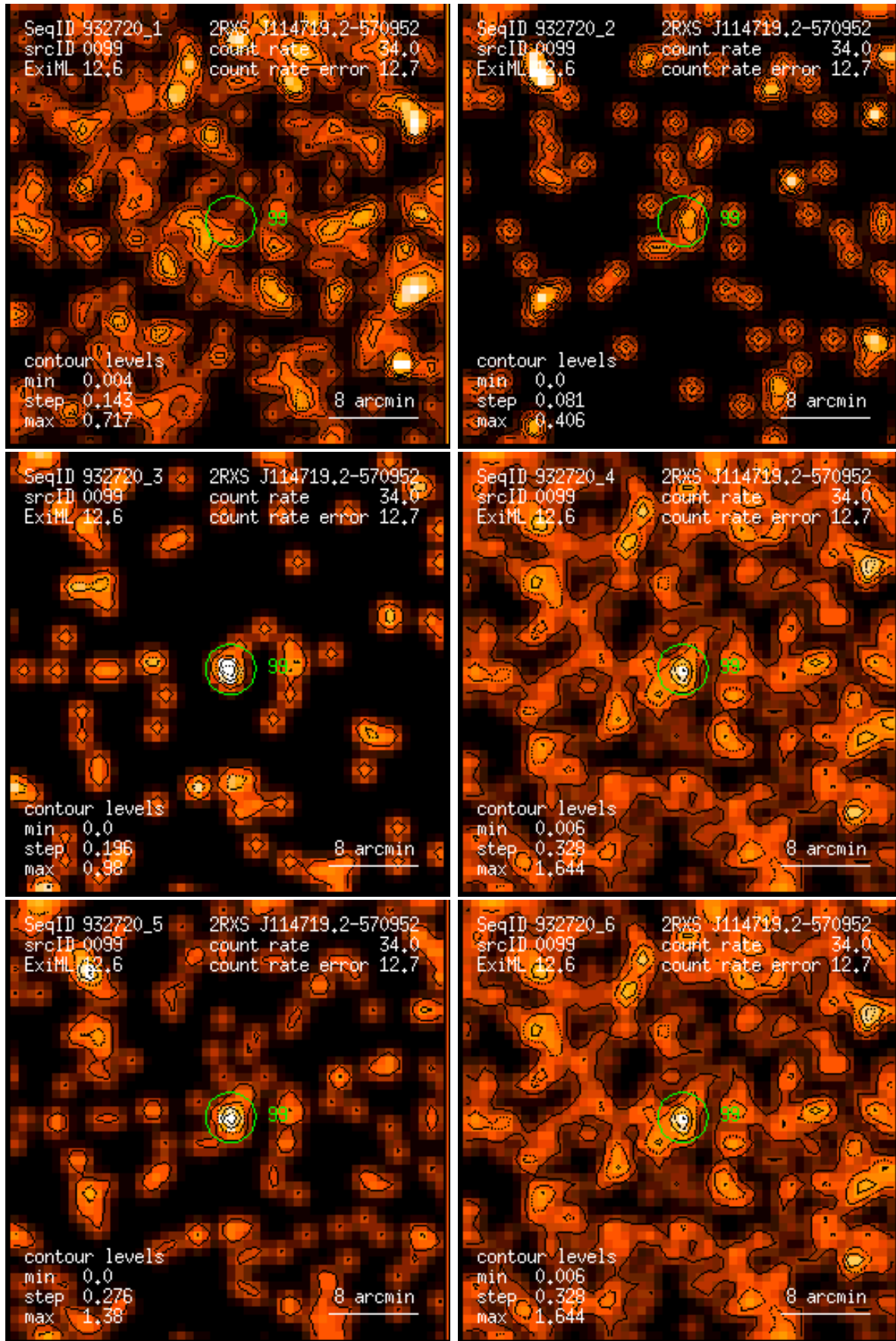
Figure 99: RASS 932720: detection 0099: band rate images, Gaussian filter: (1) PSPC channels 11 – 41, (2) 52 – 90, (3) 91 – 201, (4) 11 – 235, (5) 52 – 201, (6) 11 – 201. Broad band rates in counts/ks. Band rate contour levels in counts/ks/arcmin 2 .
