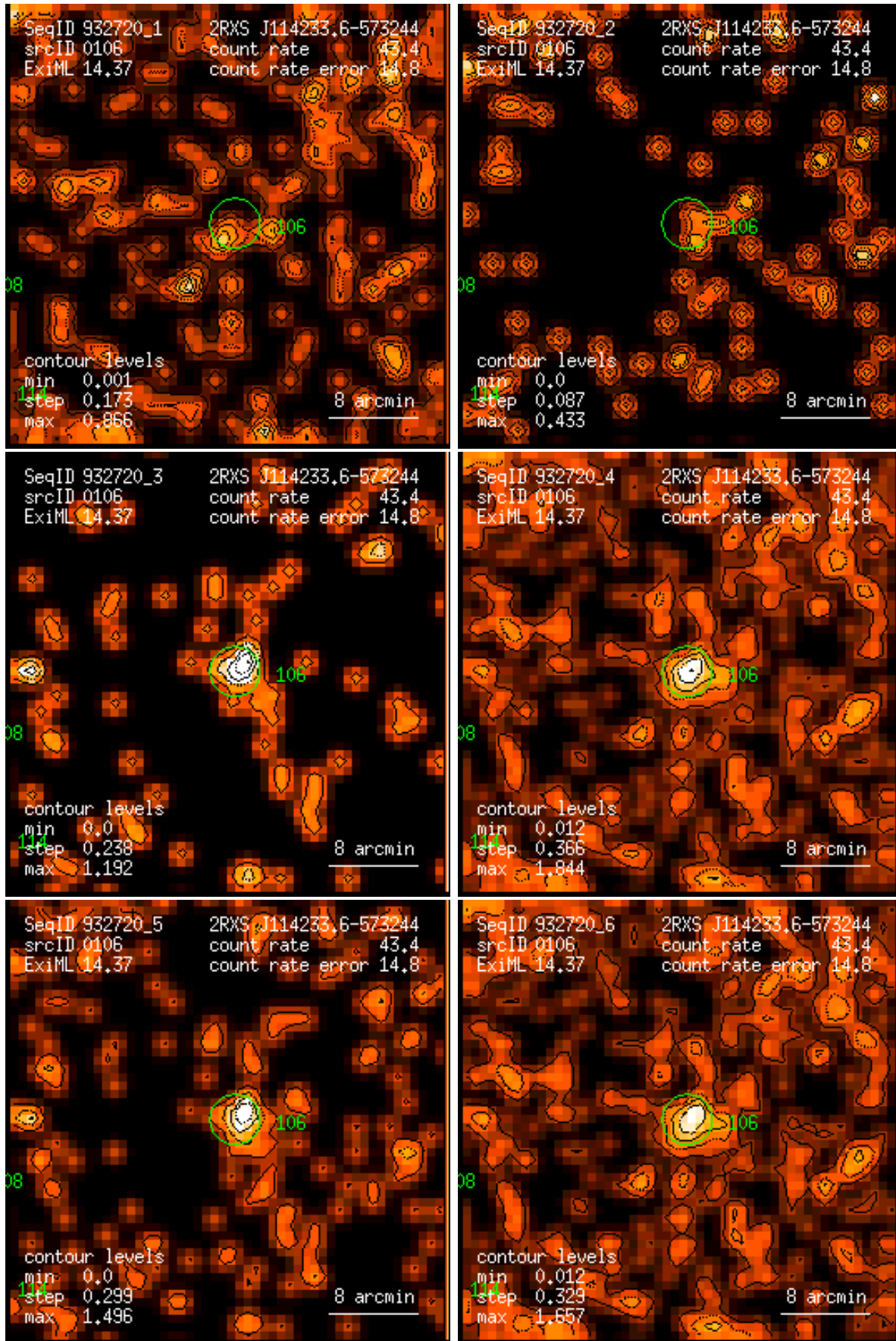
Figure 106: RASS 932720: detection 0106: band rate images, Gaussian filter: (1) PSPC channels 11 – 41, (2) 52 – 90, (3) 91 – 201, (4) 11 – 235, (5) 52 – 201, (6) 11 – 201. Broad band rates in counts/ks. Band rate contour levels in counts/ks/arcmin 2 .
