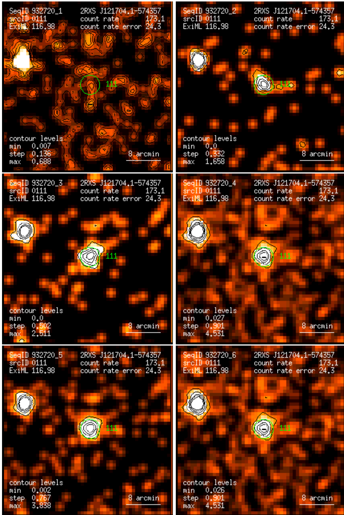
Figure 111: RASS 932720: detection 0111: band rate images, Gaussian filter: (1) PSPC channels 11 – 41, (2) 52 – 90, (3) 91 – 201, (4) 11 – 235, (5) 52 – 201, (6) 11 – 201. Broad band rates in counts/ks. Band rate contour levels in counts/ks/arcmin 2 .
