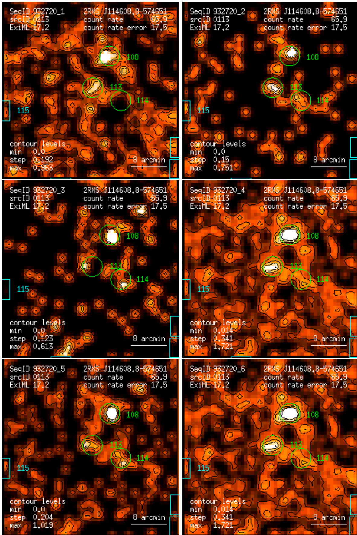
Figure 113: RASS 932720: detection 0113: band rate images, Gaussian filter: (1) PSPC channels 11 – 41, (2) 52 – 90, (3) 91 – 201, (4) 11 – 235, (5) 52 – 201, (6) 11 – 201. Broad band rates in counts/ks. Band rate contour levels in counts/ks/arcmin 2 .
