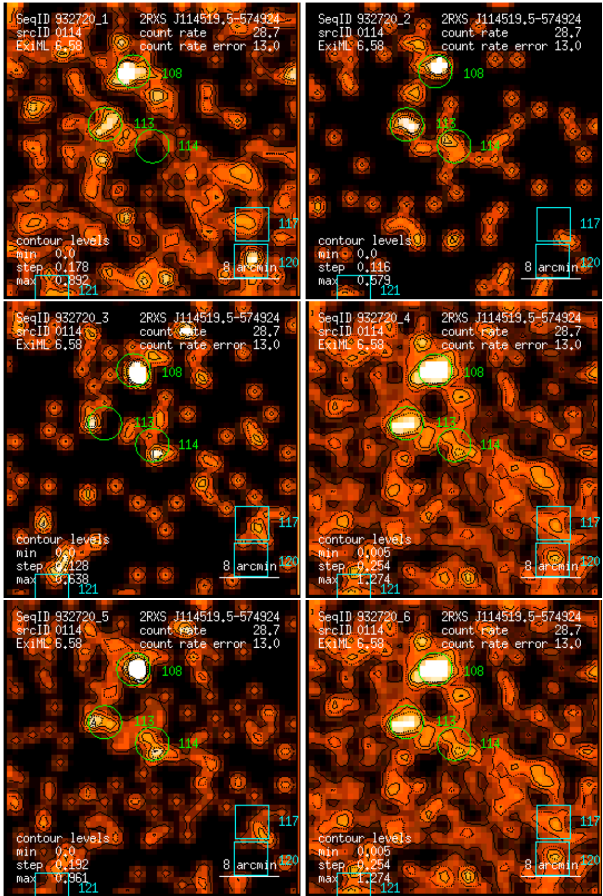
Figure 114: RASS 932720: detection 0114: band rate images, Gaussian filter: (1) PSPC channels 11 – 41, (2) 52 – 90, (3) 91 – 201, (4) 11 – 235, (5) 52 – 201, (6) 11 – 201. Broad band rates in counts/ks. Band rate contour levels in counts/ks/arcmin 2 .
