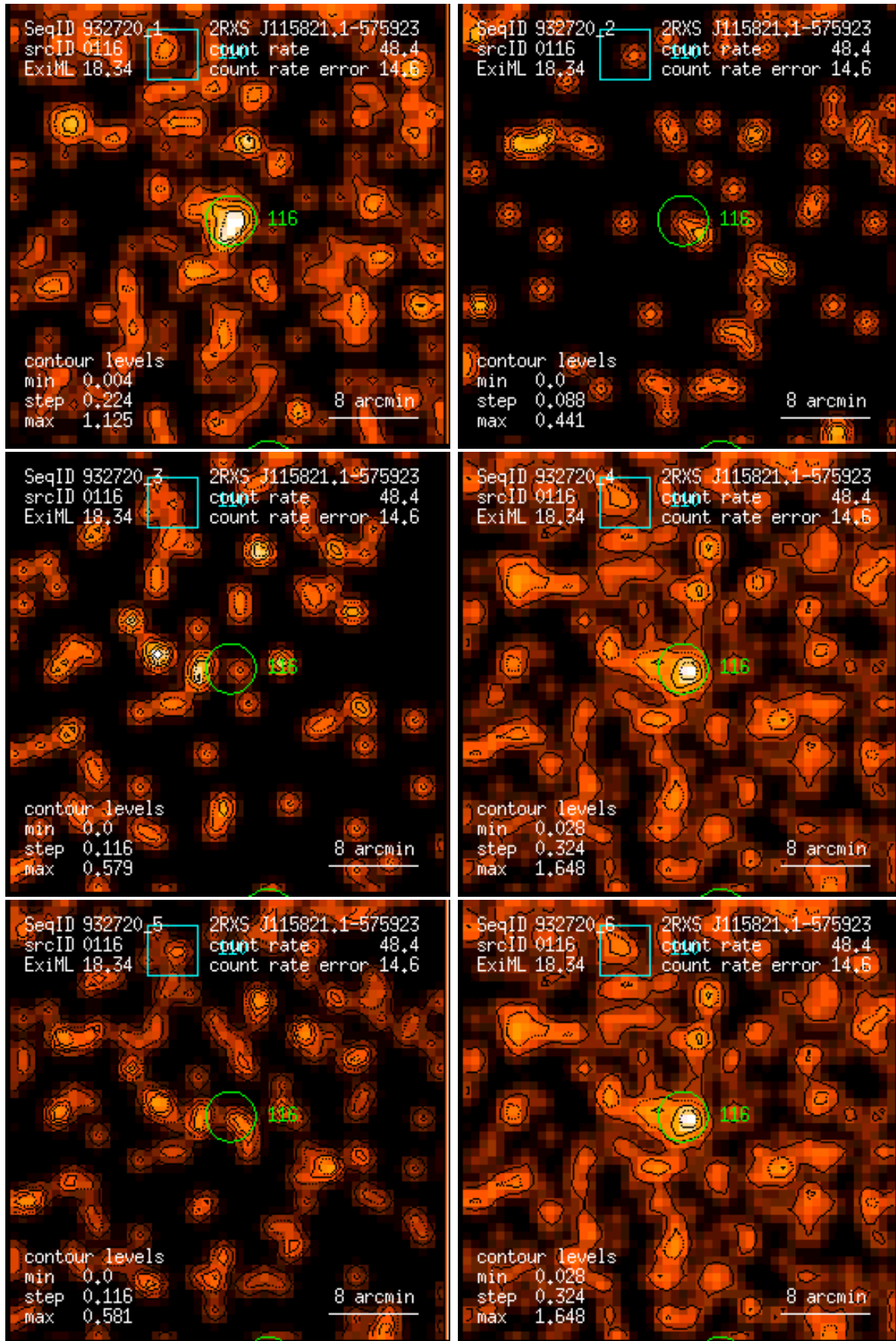
Figure 116: RASS 932720: detection 0116: band rate images, Gaussian filter: (1) PSPC channels 11 – 41, (2) 52 – 90, (3) 91 – 201, (4) 11 – 235, (5) 52 – 201, (6) 11 – 201. Broad band rates in counts/ks. Band rate contour levels in counts/ks/arcmin 2 .
