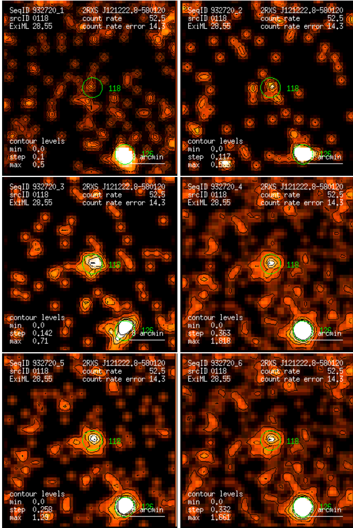
Figure 118: RASS 932720: detection 0118: band rate images, Gaussian filter: (1) PSPC channels 11 – 41, (2) 52 – 90, (3) 91 – 201, (4) 11 – 235, (5) 52 – 201, (6) 11 – 201. Broad band rates in counts/ks. Band rate contour levels in counts/ks/arcmin 2 .
