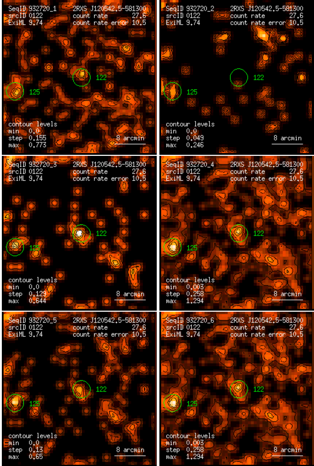
Figure 122: RASS 932720: detection 0122: band rate images, Gaussian filter: (1) PSPC channels 11 – 41, (2) 52 – 90, (3) 91 – 201, (4) 11 – 235, (5) 52 – 201, (6) 11 – 201. Broad band rates in counts/ks. Band rate contour levels in counts/ks/arcmin 2 .
