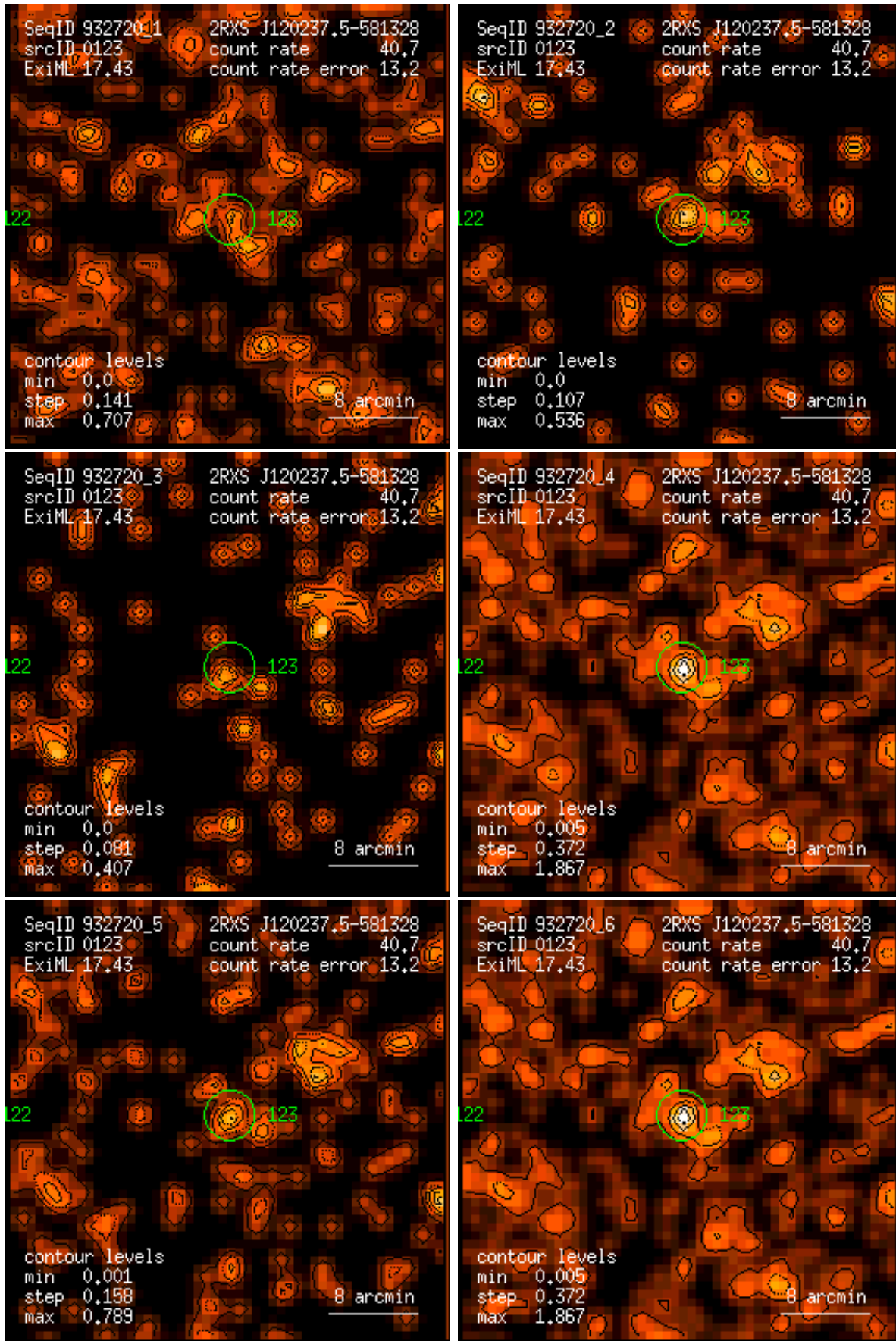
Figure 123: RASS 932720: detection 0123: band rate images, Gaussian filter: (1) PSPC channels 11 – 41, (2) 52 – 90, (3) 91 – 201, (4) 11 – 235, (5) 52 – 201, (6) 11 – 201. Broad band rates in counts/ks. Band rate contour levels in counts/ks/arcmin 2 .
