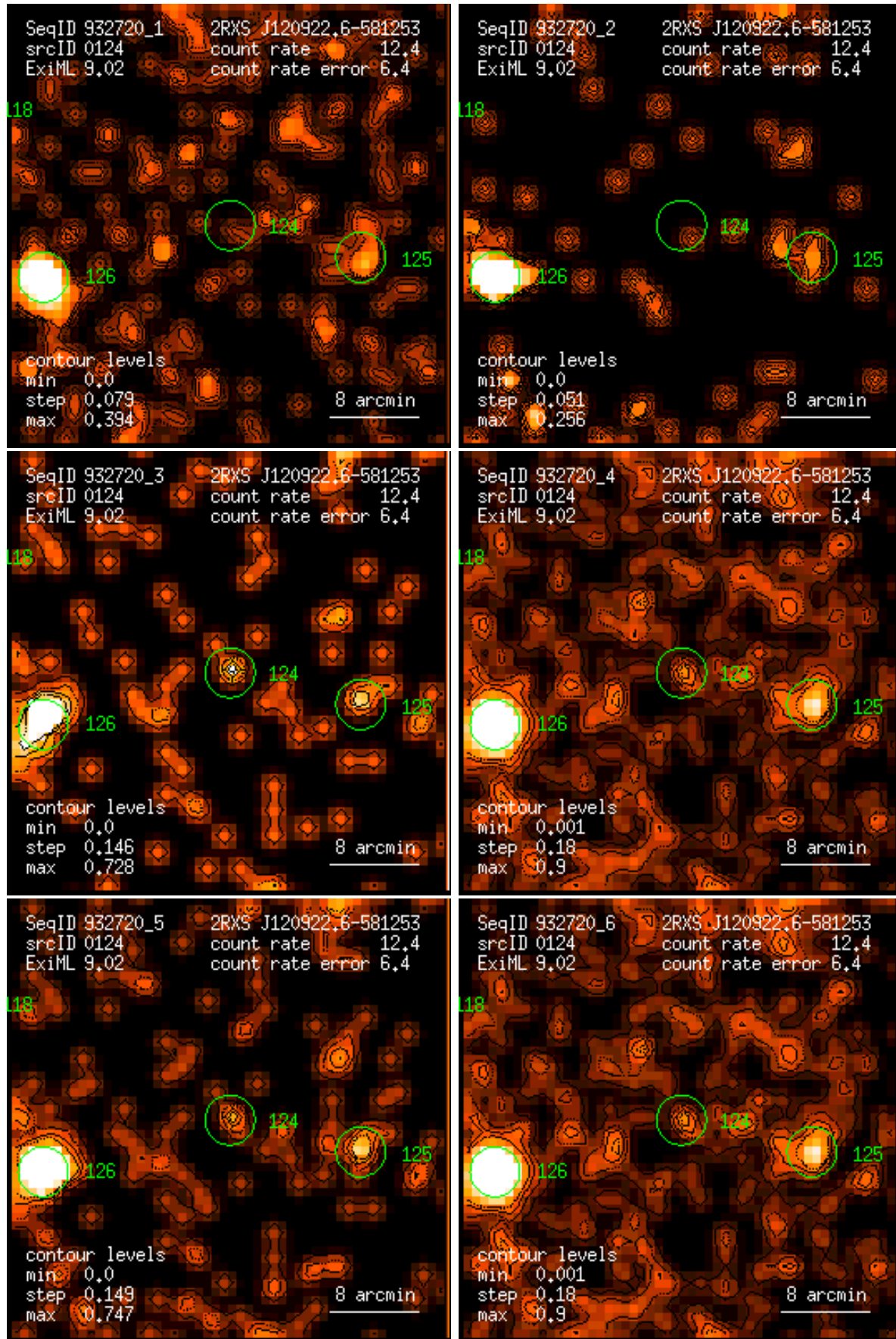
Figure 124: RASS 932720: detection 0124: band rate images, Gaussian filter: (1) PSPC channels 11 – 41, (2) 52 – 90, (3) 91 – 201, (4) 11 – 235, (5) 52 – 201, (6) 11 – 201. Broad band rates in counts/ks. Band rate contour levels in counts/ks/arcmin 2 .
