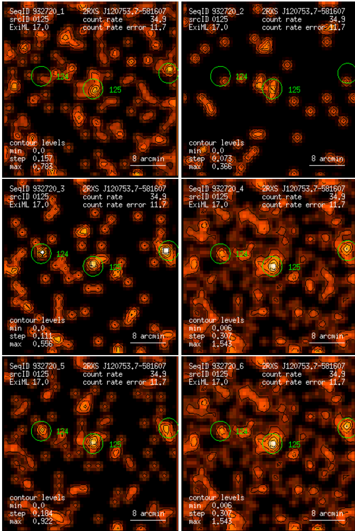
Figure 125: RASS 932720: detection 0125: band rate images, Gaussian filter: (1) PSPC channels 11 – 41, (2) 52 – 90, (3) 91 – 201, (4) 11 – 235, (5) 52 – 201, (6) 11 – 201. Broad band rates in counts/ks. Band rate contour levels in counts/ks/arcmin 2 .
