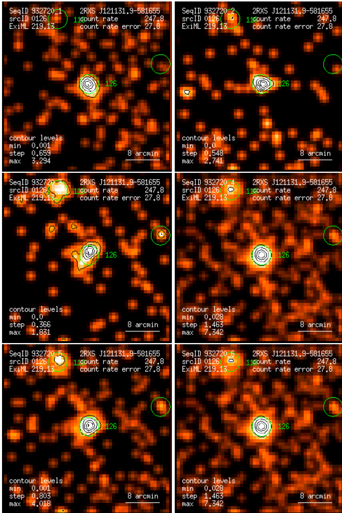
Figure 126: RASS 932720: detection 0126: band rate images, Gaussian filter: (1) PSPC channels 11 – 41, (2) 52 – 90, (3) 91 – 201, (4) 11 – 235, (5) 52 – 201, (6) 11 – 201. Broad band rates in counts/ks. Band rate contour levels in counts/ks/arcmin 2 .
