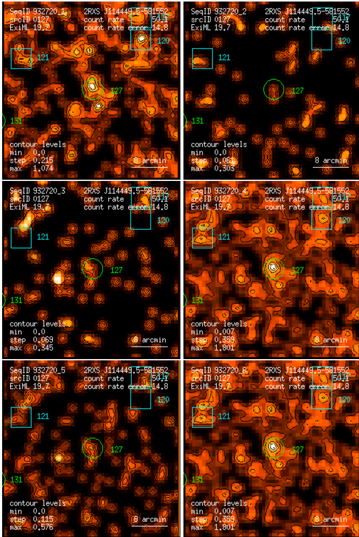
Figure 127: RASS 932720: detection 0127: band rate images, Gaussian filter: (1) PSPC channels 11 – 41, (2) 52 – 90, (3) 91 – 201, (4) 11 – 235, (5) 52 – 201, (6) 11 – 201. Broad band rates in counts/ks. Band rate contour levels in counts/ks/arcmin 2 .
