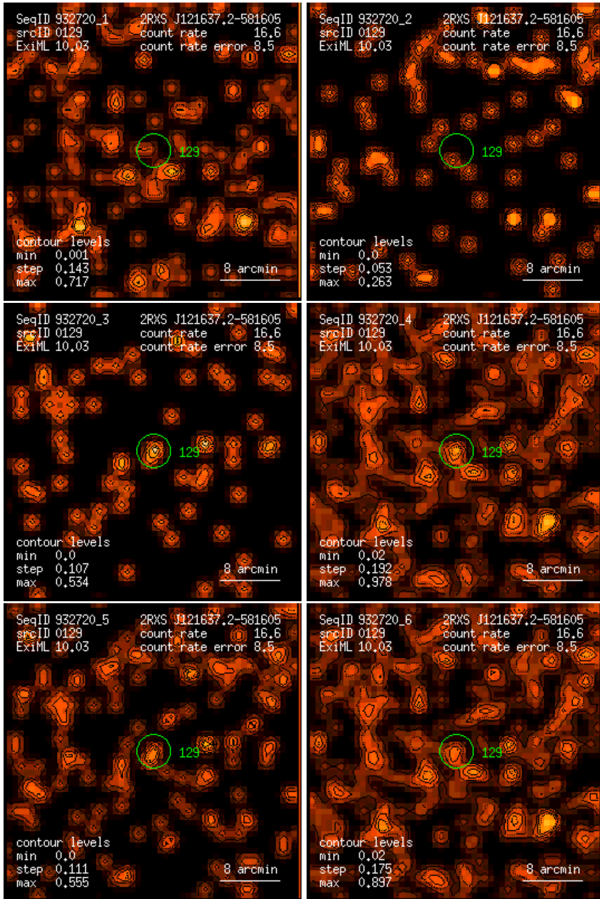
Figure 129: RASS 932720: detection 0129: band rate images, Gaussian filter: (1) PSPC channels 11 – 41, (2) 52 – 90, (3) 91 – 201, (4) 11 – 235, (5) 52 – 201, (6) 11 – 201. Broad band rates in counts/ks. Band rate contour levels in counts/ks/arcmin 2 .
