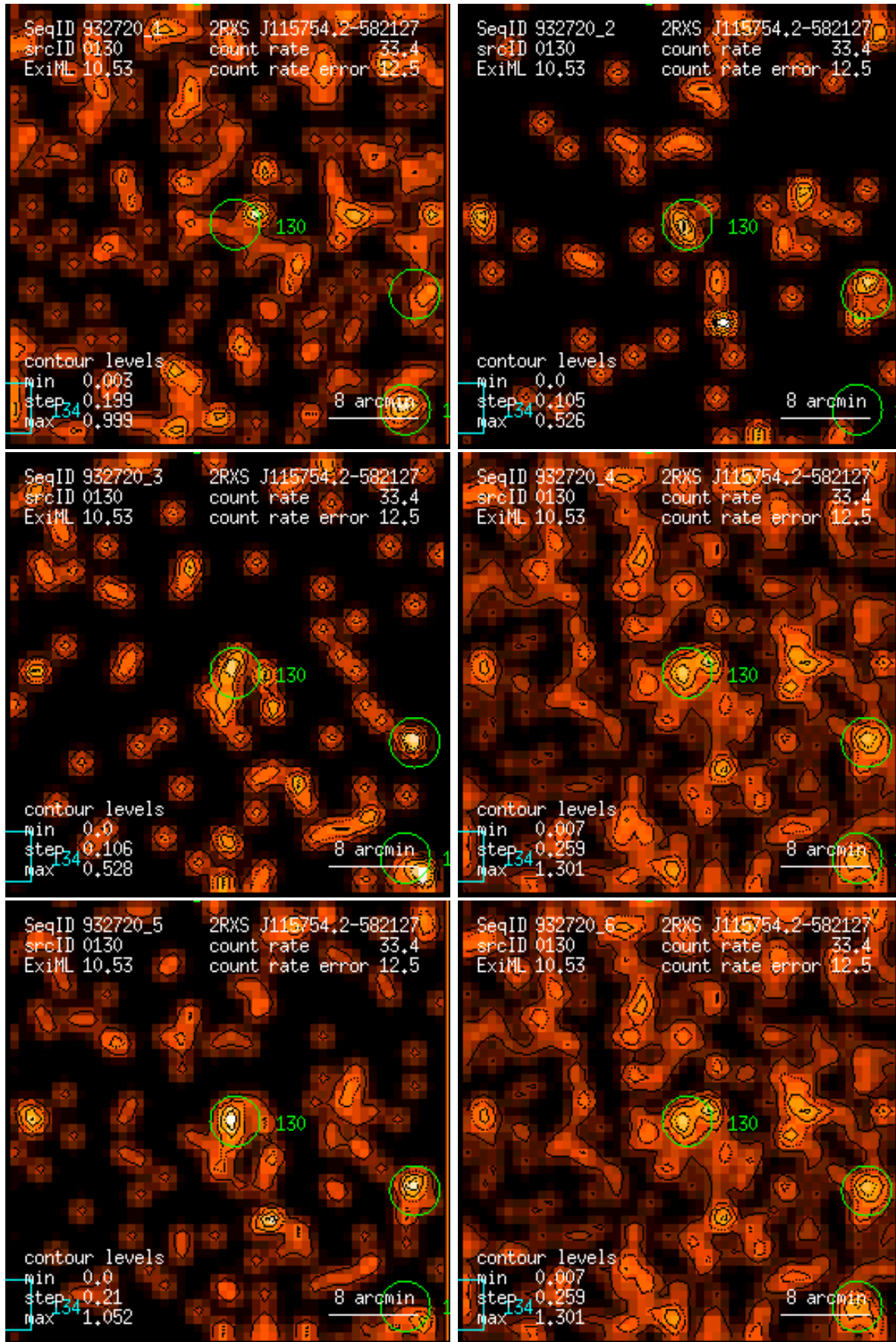
Figure 130: RASS 932720: detection 0130: band rate images, Gaussian filter: (1) PSPC channels 11 – 41, (2) 52 – 90, (3) 91 – 201, (4) 11 – 235, (5) 52 – 201, (6) 11 – 201. Broad band rates in counts/ks. Band rate contour levels in counts/ks/arcmin 2 .
