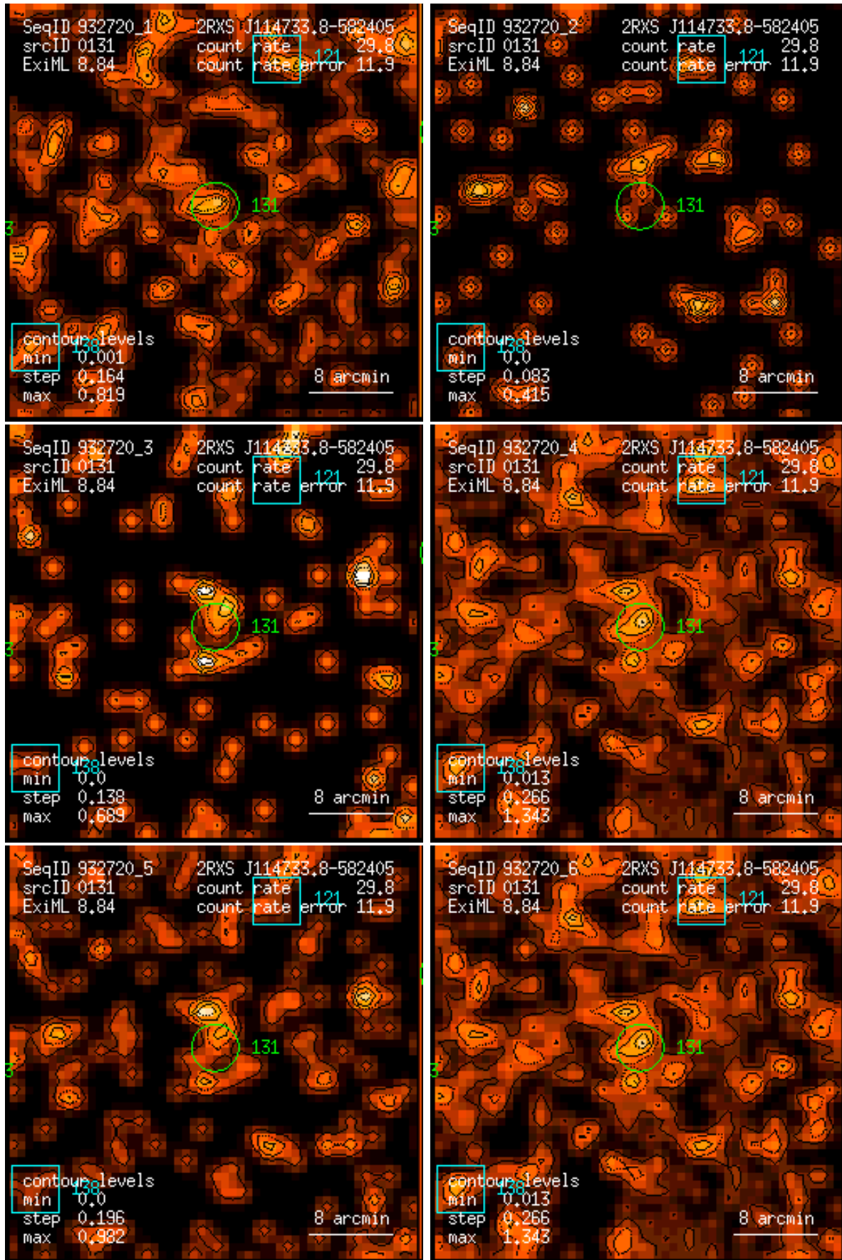
Figure 131: RASS 932720: detection 0131: band rate images, Gaussian filter: (1) PSPC channels 11 – 41, (2) 52 – 90, (3) 91 – 201, (4) 11 – 235, (5) 52 – 201, (6) 11 – 201. Broad band rates in counts/ks. Band rate contour levels in counts/ks/arcmin 2 .
