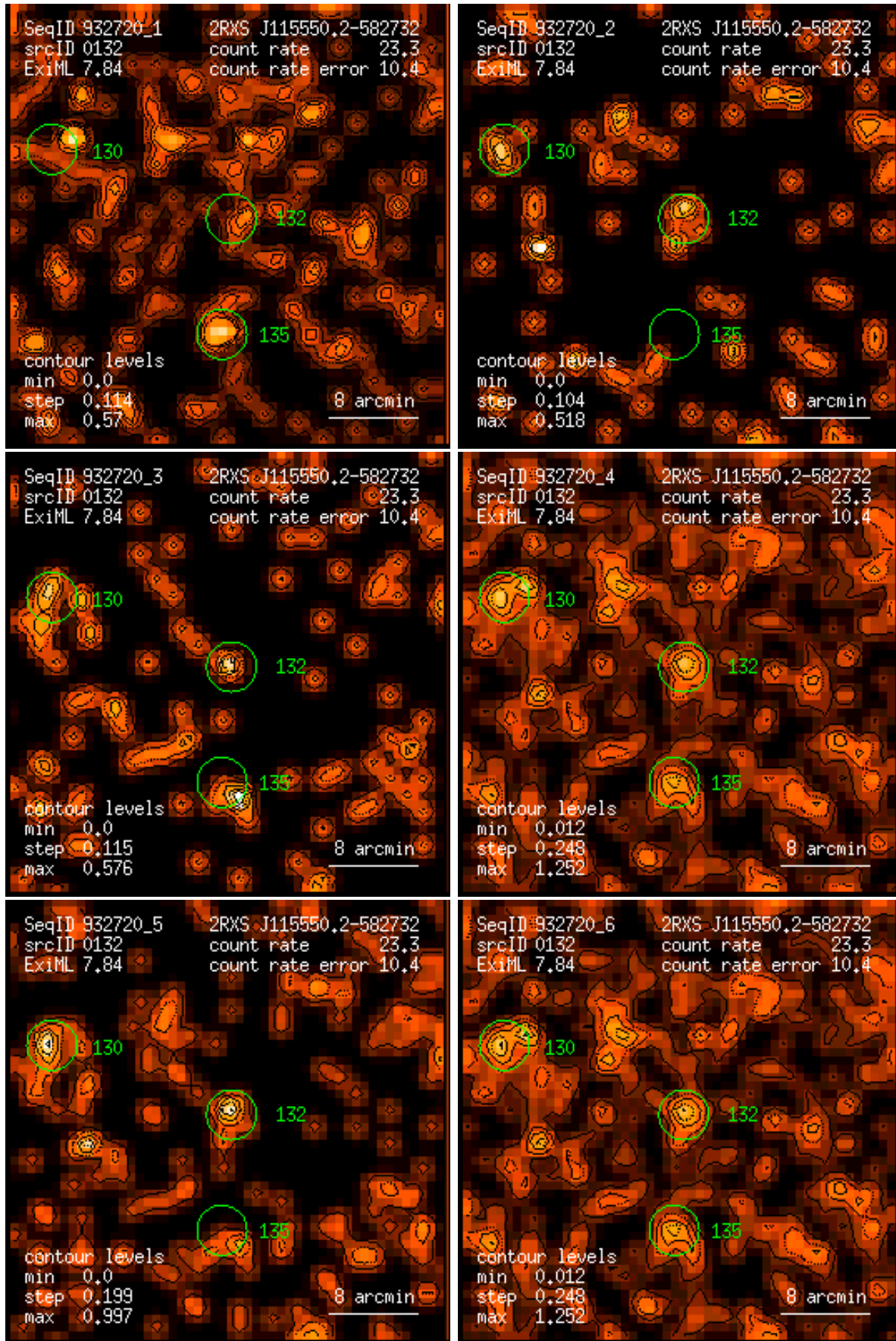
Figure 132: RASS 932720: detection 0132: band rate images, Gaussian filter: (1) PSPC channels 11 – 41, (2) 52 – 90, (3) 91 – 201, (4) 11 – 235, (5) 52 – 201, (6) 11 – 201. Broad band rates in counts/ks. Band rate contour levels in counts/ks/arcmin 2 .
