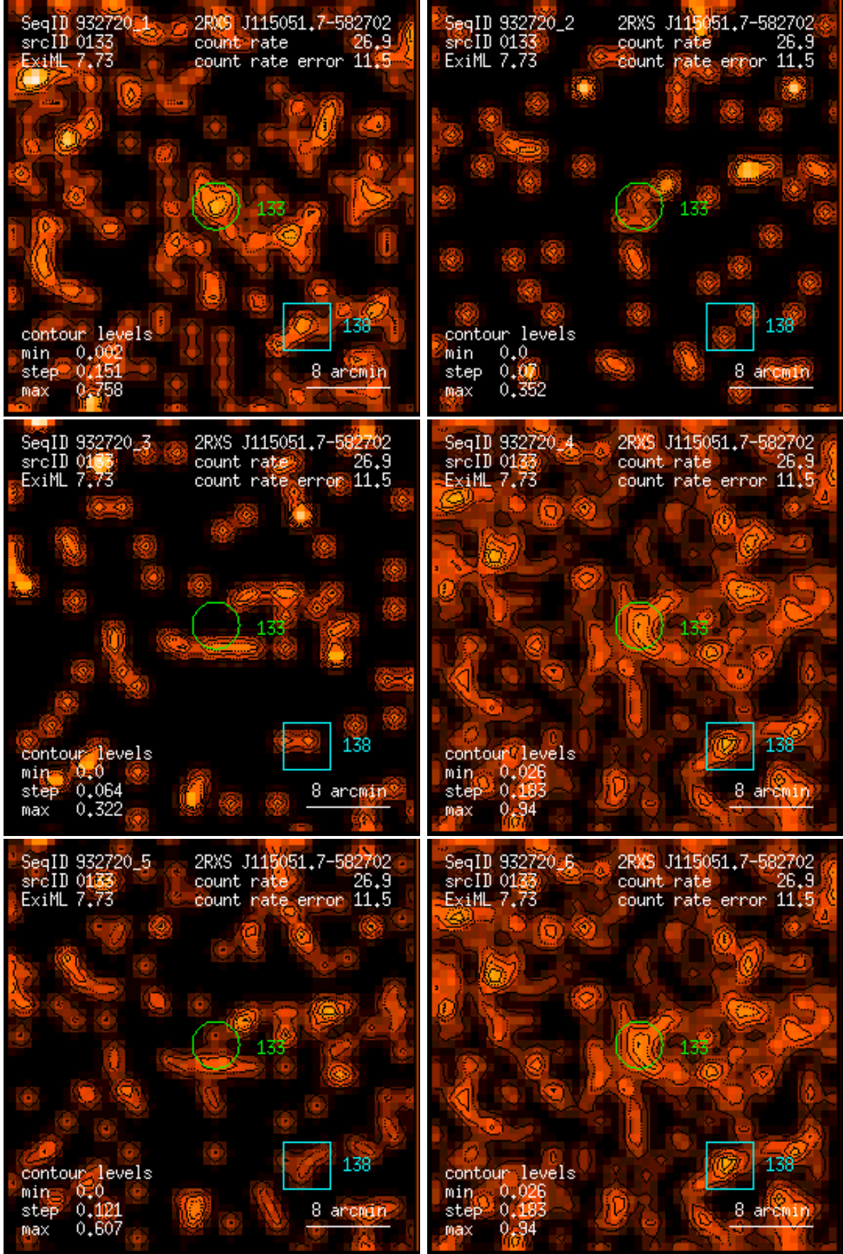
Figure 133: RASS 932720: detection 0133: band rate images, Gaussian filter: (1) PSPC channels 11 – 41, (2) 52 – 90, (3) 91 – 201, (4) 11 – 235, (5) 52 – 201, (6) 11 – 201. Broad band rates in counts/ks. Band rate contour levels in counts/ks/arcmin 2 .
