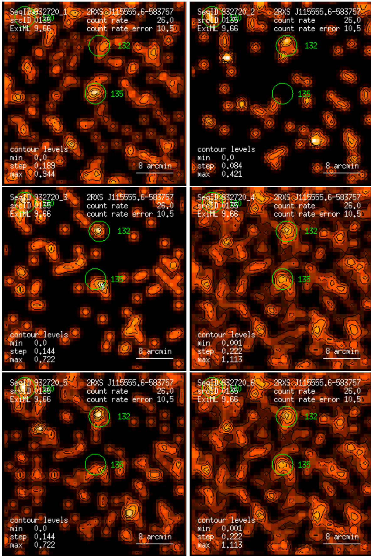
Figure 135: RASS 932720: detection 0135: band rate images, Gaussian filter: (1) PSPC channels 11 – 41, (2) 52 – 90, (3) 91 – 201, (4) 11 – 235, (5) 52 – 201, (6) 11 – 201. Broad band rates in counts/ks. Band rate contour levels in counts/ks/arcmin 2 .
