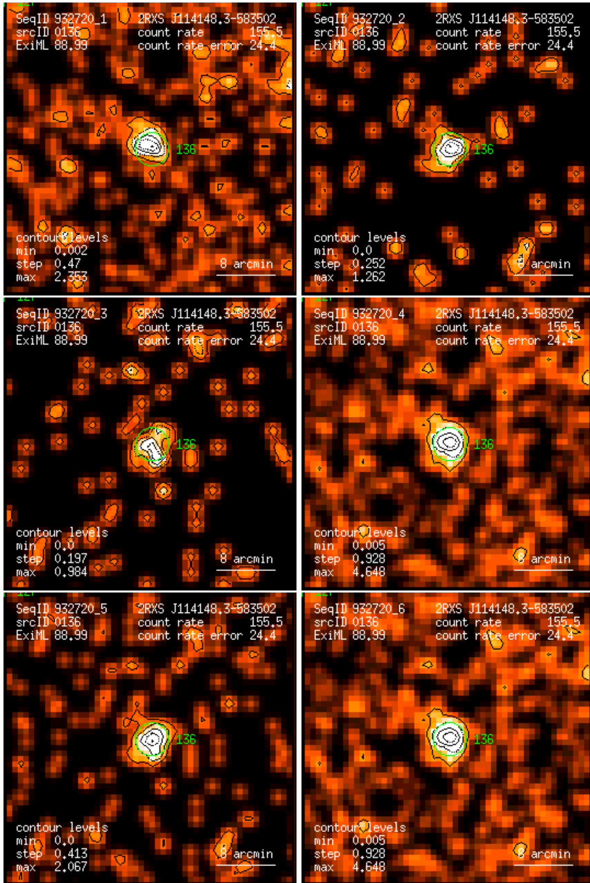
Figure 136: RASS 932720: detection 0136: band rate images, Gaussian filter: (1) PSPC channels 11 – 41, (2) 52 – 90, (3) 91 – 201, (4) 11 – 235, (5) 52 – 201, (6) 11 – 201. Broad band rates in counts/ks. Band rate contour levels in counts/ks/arcmin 2 .
