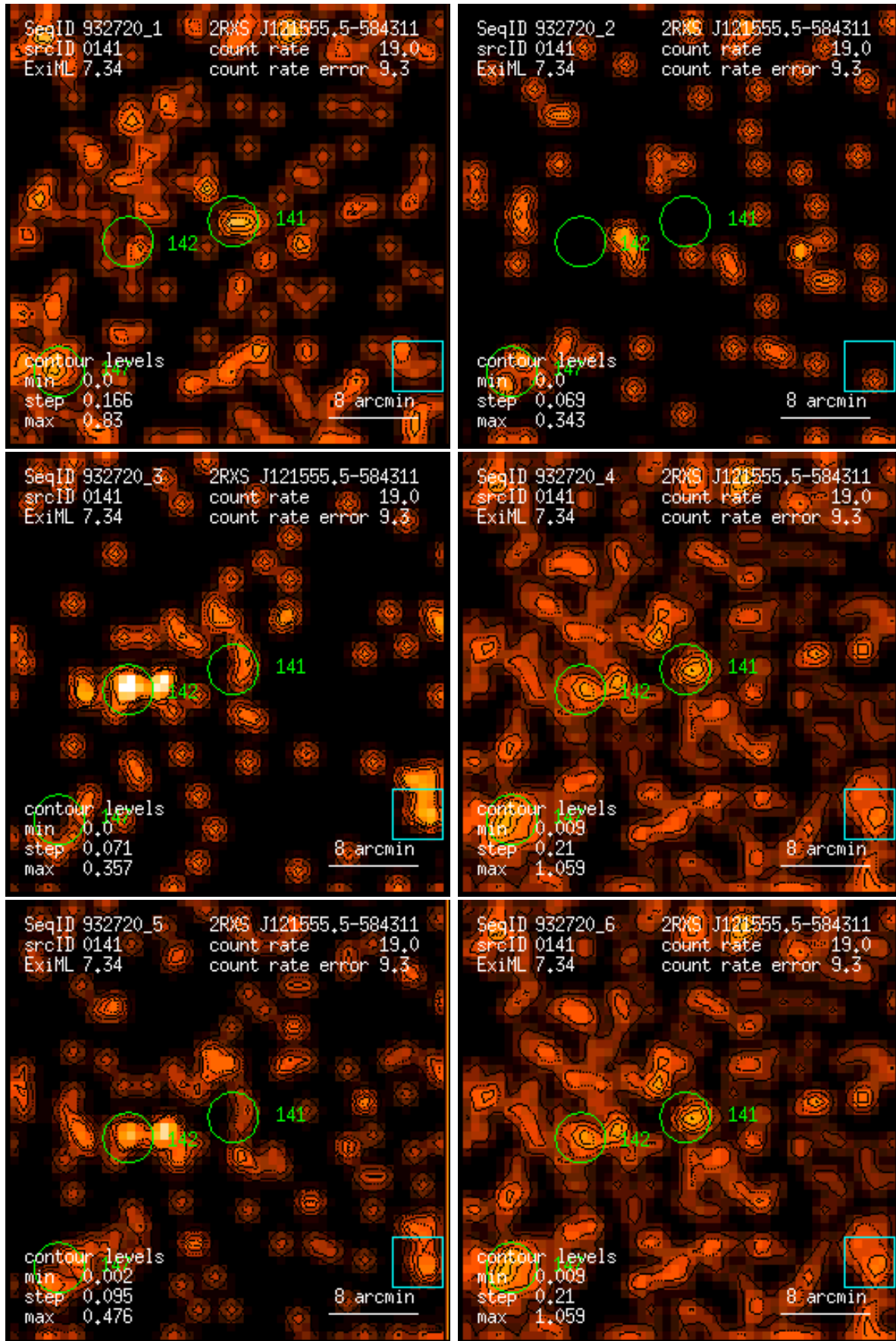
Figure 141: RASS 932720: detection 0141: band rate images, Gaussian filter: (1) PSPC channels 11 – 41, (2) 52 – 90, (3) 91 – 201, (4) 11 – 235, (5) 52 – 201, (6) 11 – 201. Broad band rates in counts/ks. Band rate contour levels in counts/ks/arcmin 2 .
