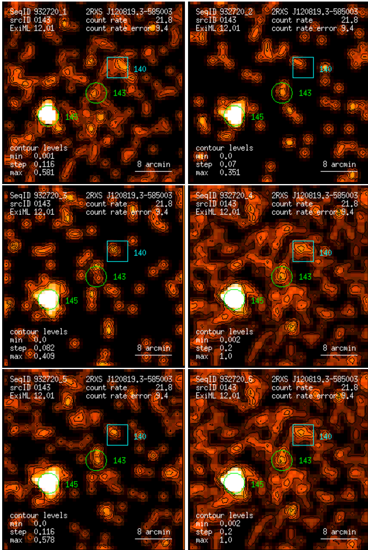
Figure 143: RASS 932720: detection 0143: band rate images, Gaussian filter: (1) PSPC channels 11 – 41, (2) 52 – 90, (3) 91 – 201, (4) 11 – 235, (5) 52 – 201, (6) 11 – 201. Broad band rates in counts/ks. Band rate contour levels in counts/ks/arcmin 2 .
