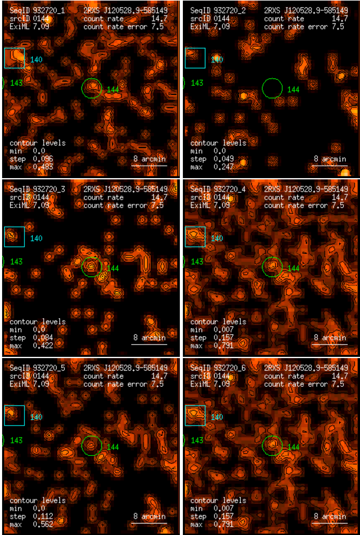
Figure 144: RASS 932720: detection 0144: band rate images, Gaussian filter: (1) PSPC channels 11 – 41, (2) 52 – 90, (3) 91 – 201, (4) 11 – 235, (5) 52 – 201, (6) 11 – 201. Broad band rates in counts/ks. Band rate contour levels in counts/ks/arcmin 2 .
