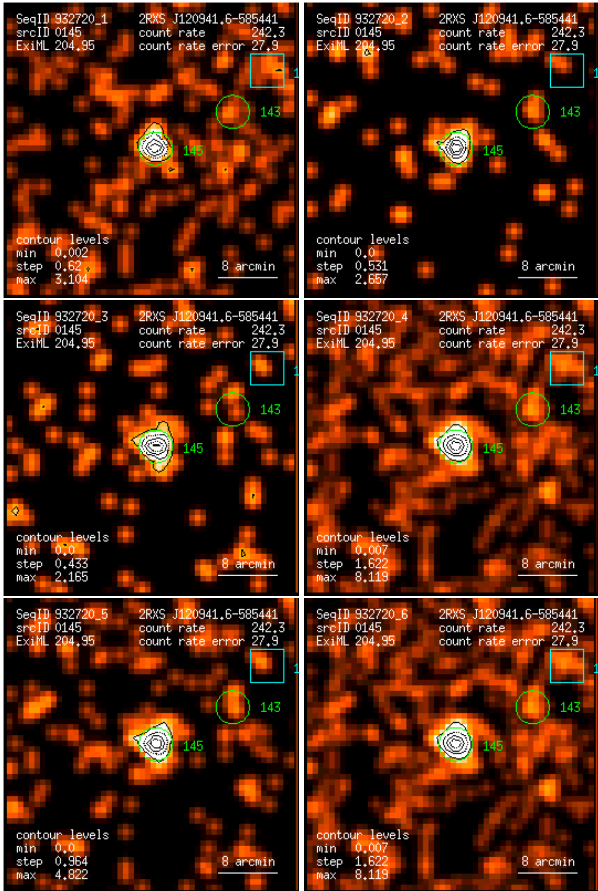
Figure 145: RASS 932720: detection 0145: band rate images, Gaussian filter: (1) PSPC channels 11 – 41, (2) 52 – 90, (3) 91 – 201, (4) 11 – 235, (5) 52 – 201, (6) 11 – 201. Broad band rates in counts/ks. Band rate contour levels in counts/ks/arcmin 2 .
