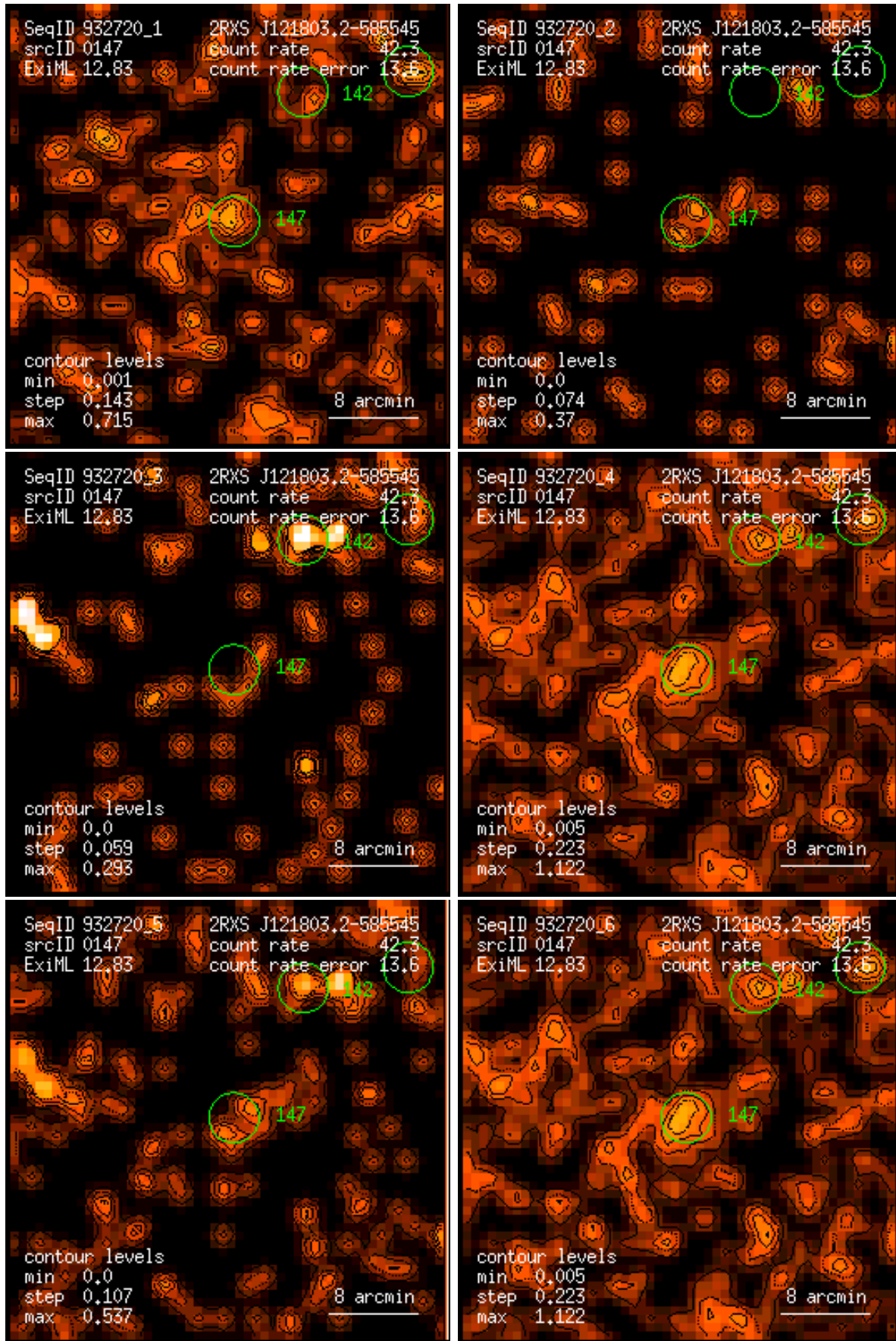
Figure 147: RASS 932720: detection 0147: band rate images, Gaussian filter: (1) PSPC channels 11 – 41, (2) 52 – 90, (3) 91 – 201, (4) 11 – 235, (5) 52 – 201, (6) 11 – 201. Broad band rates in counts/ks. Band rate contour levels in counts/ks/arcmin 2 .
