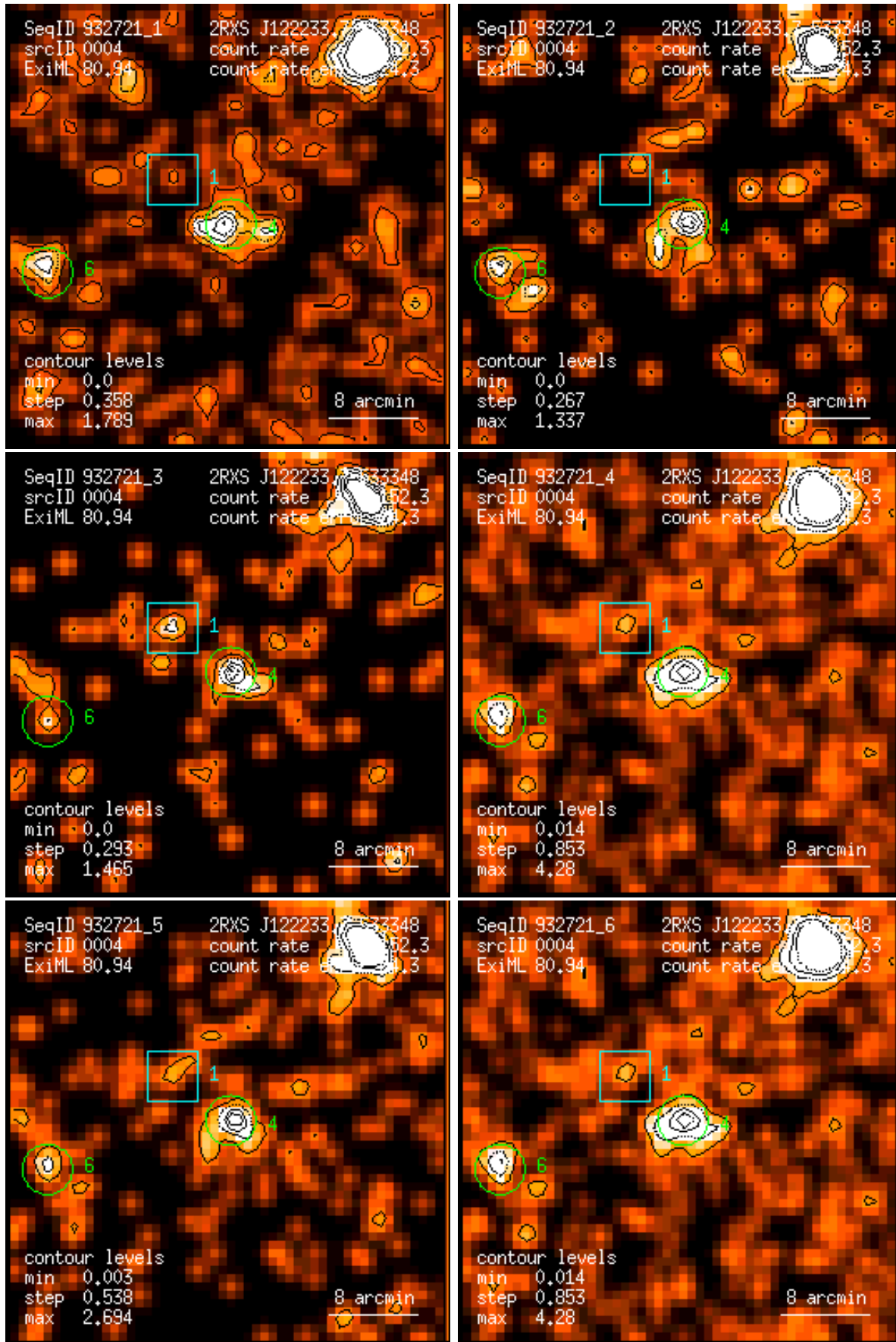
Figure 4: RASS 932721: detection 0004: band rate images, Gaussian filter: (1) PSPC channels 11 – 41, (2) 52 – 90, (3) 91 – 201, (4) 11 – 235, (5) 52 – 201, (6) 11 – 201. Broad band rates in counts/ks. Band rate contour levels in counts/ks/arcmin 2 .
