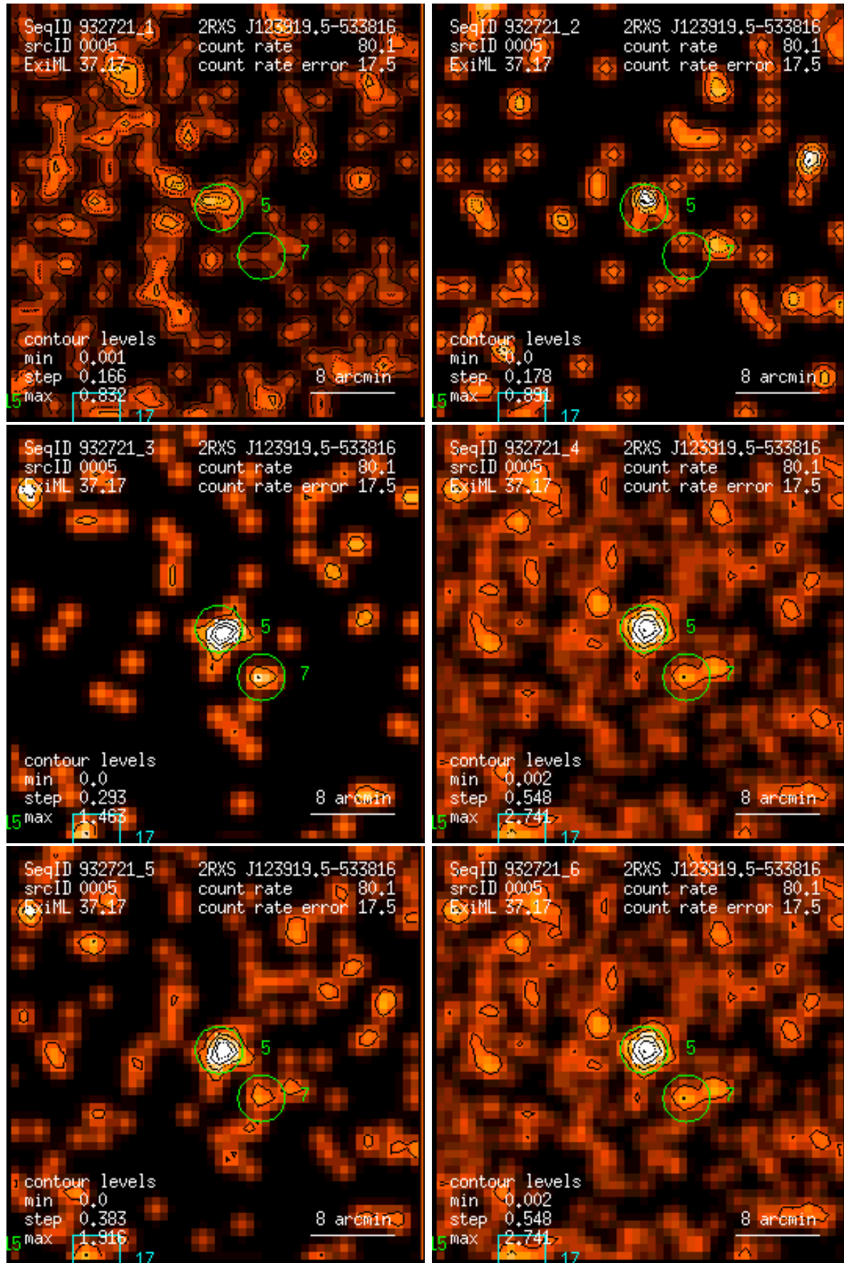
Figure 5: RASS 932721: detection 0005: band rate images, Gaussian filter: (1) PSPC channels 11 – 41, (2) 52 – 90, (3) 91 – 201, (4) 11 – 235, (5) 52 – 201, (6) 11 – 201. Broad band rates in counts/ks. Band rate contour levels in counts/ks/arcmin 2 .
