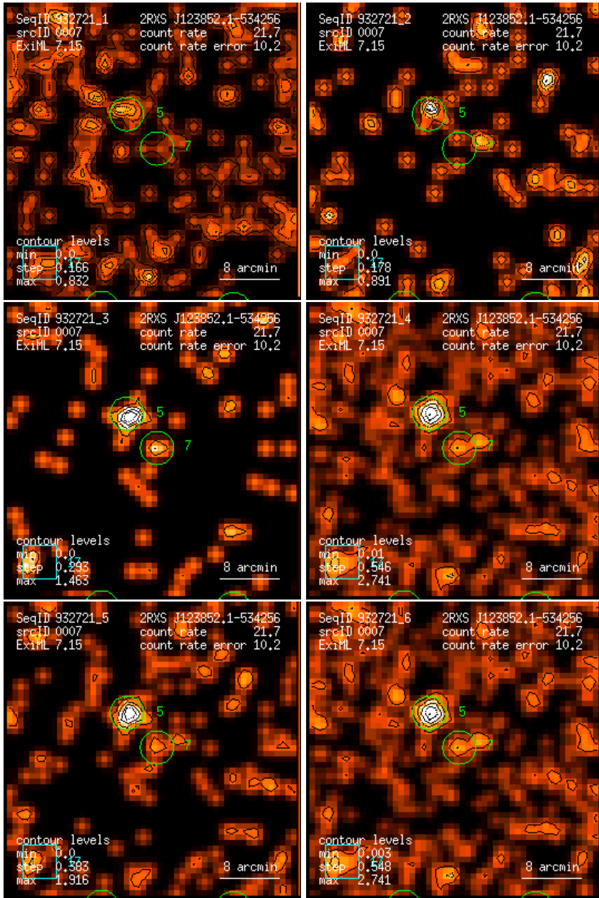
Figure 7: RASS 932721: detection 0007: band rate images, Gaussian filter: (1) PSPC channels 11 – 41, (2) 52 – 90, (3) 91 – 201, (4) 11 – 235, (5) 52 – 201, (6) 11 – 201. Broad band rates in counts/ks. Band rate contour levels in counts/ks/arcmin 2 .
