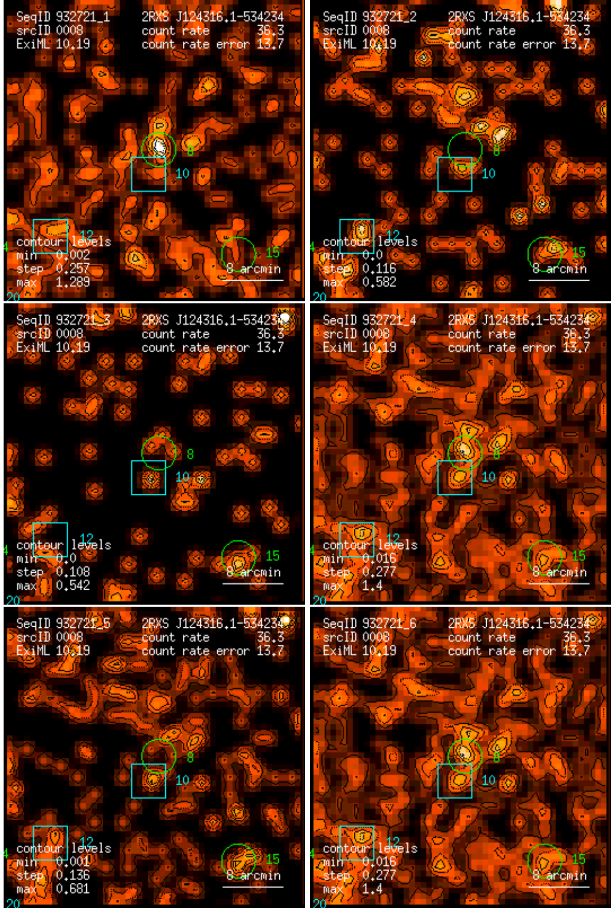
Figure 8: RASS 932721: detection 0008: band rate images, Gaussian filter: (1) PSPC channels 11 – 41, (2) 52 – 90, (3) 91 – 201, (4) 11 – 235, (5) 52 – 201, (6) 11 – 201. Broad band rates in counts/ks. Band rate contour levels in counts/ks/arcmin 2 .
