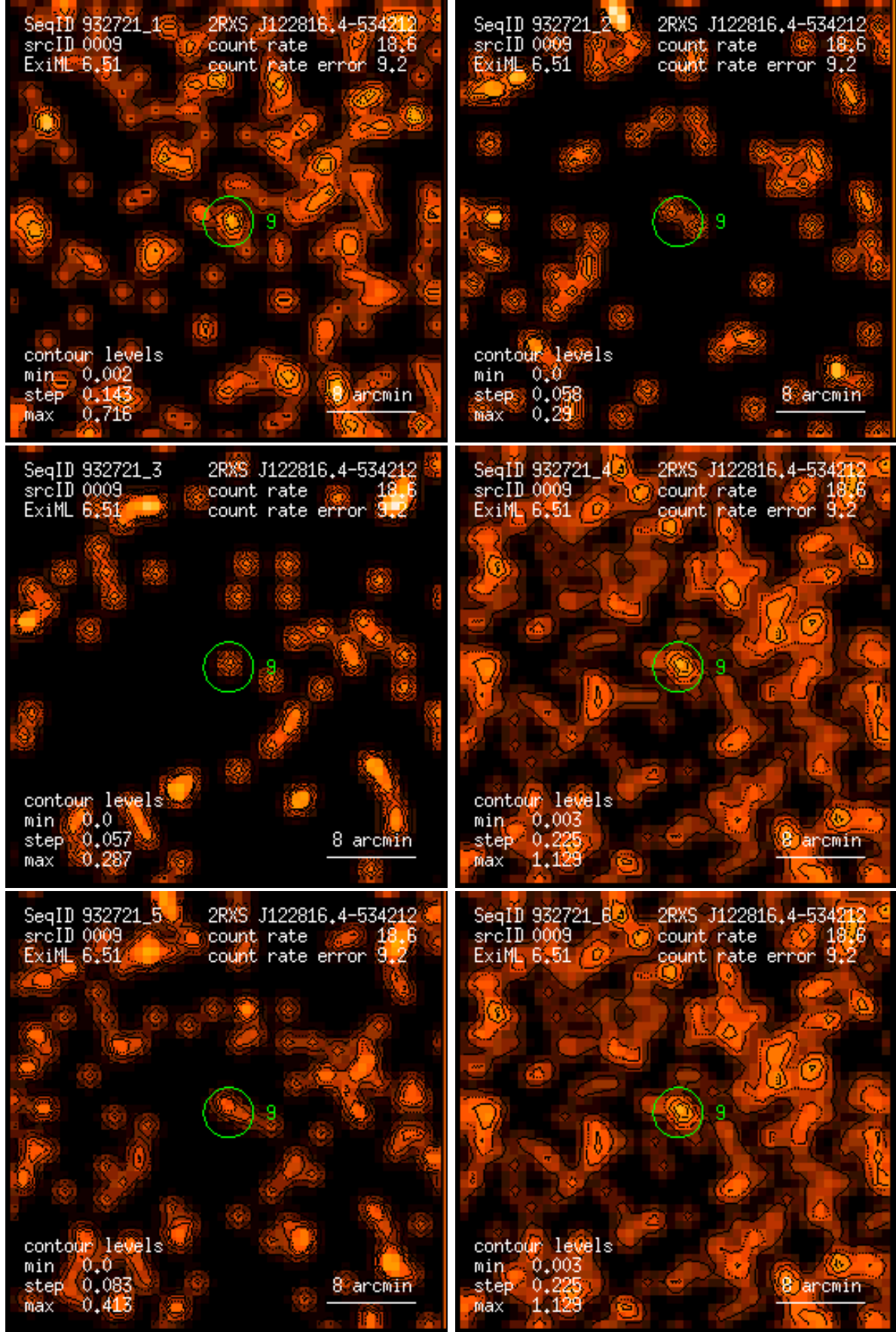
Figure 9: RASS 932721: detection 0009: band rate images, Gaussian filter: (1) PSPC channels 11 – 41, (2) 52 – 90, (3) 91 – 201, (4) 11 – 235, (5) 52 – 201, (6) 11 – 201. Broad band rates in counts/ks. Band rate contour levels in counts/ks/arcmin 2 .
