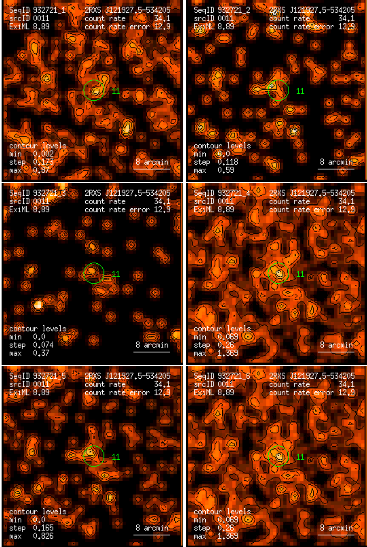
Figure 11: RASS 932721: detection 0011: band rate images, Gaussian filter: (1) PSPC channels 11 – 41, (2) 52 – 90, (3) 91 – 201, (4) 11 – 235, (5) 52 – 201, (6) 11 – 201. Broad band rates in counts/ks. Band rate contour levels in counts/ks/arcmin 2 .
