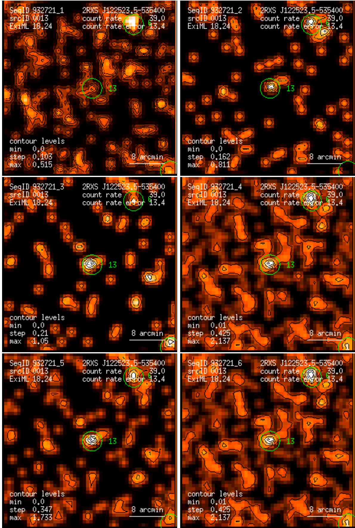
Figure 13: RASS 932721: detection 0013: band rate images, Gaussian filter: (1) PSPC channels 11 – 41, (2) 52 – 90, (3) 91 – 201, (4) 11 – 235, (5) 52 – 201, (6) 11 – 201. Broad band rates in counts/ks. Band rate contour levels in counts/ks/arcmin 2 .
