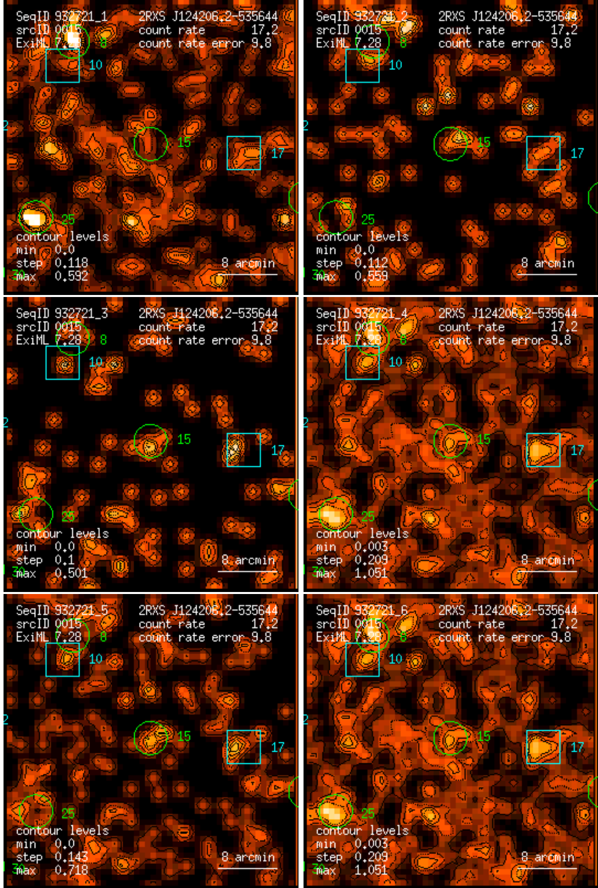
Figure 15: RASS 932721: detection 0015: band rate images, Gaussian filter: (1) PSPC channels 11 – 41, (2) 52 – 90, (3) 91 – 201, (4) 11 – 235, (5) 52 – 201, (6) 11 – 201. Broad band rates in counts/ks. Band rate contour levels in counts/ks/arcmin 2 .
