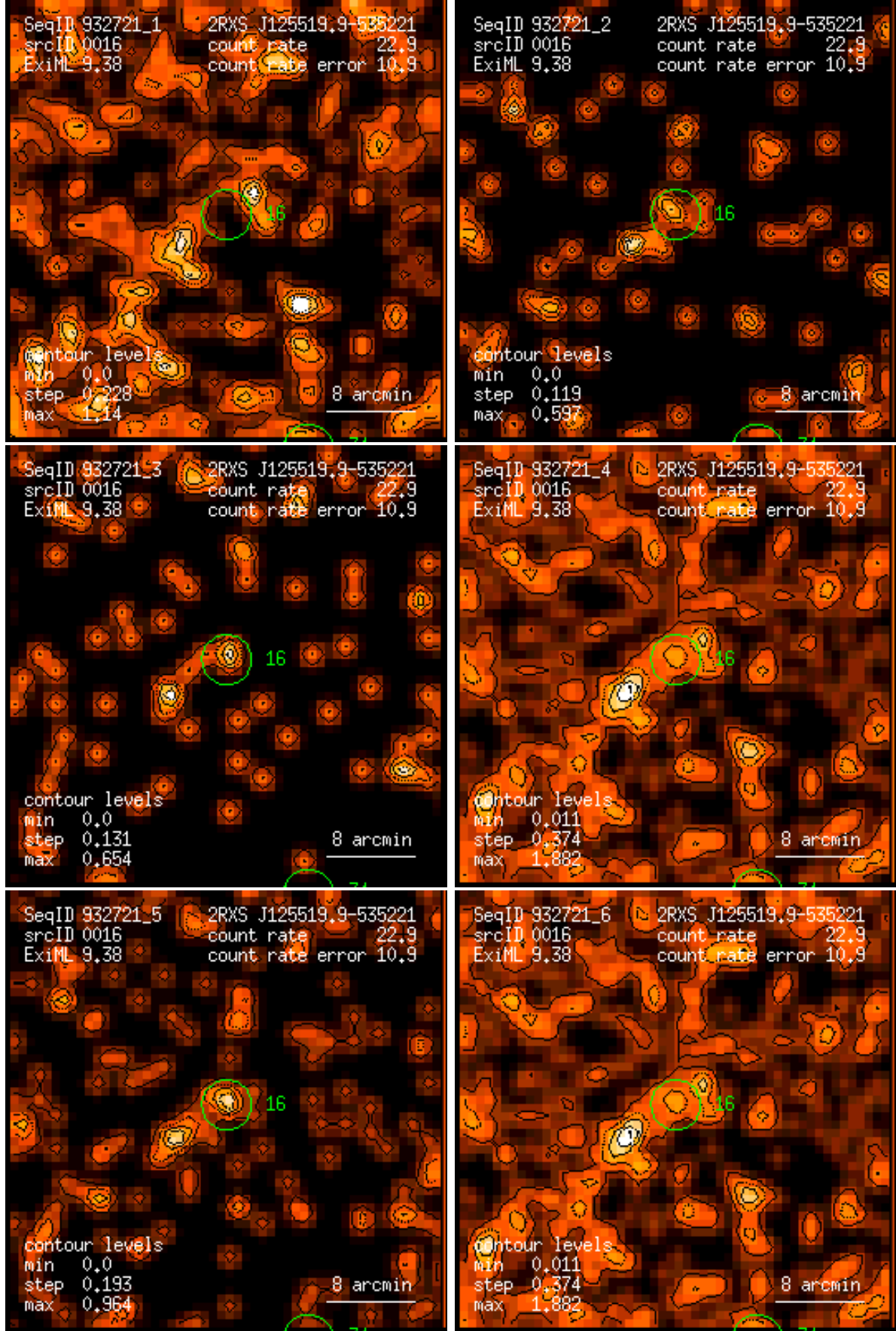
Figure 16: RASS 932721: detection 0016: band rate images, Gaussian filter: (1) PSPC channels 11 – 41, (2) 52 – 90, (3) 91 – 201, (4) 11 – 235, (5) 52 – 201, (6) 11 – 201. Broad band rates in counts/ks. Band rate contour levels in counts/ks/arcmin 2 .
