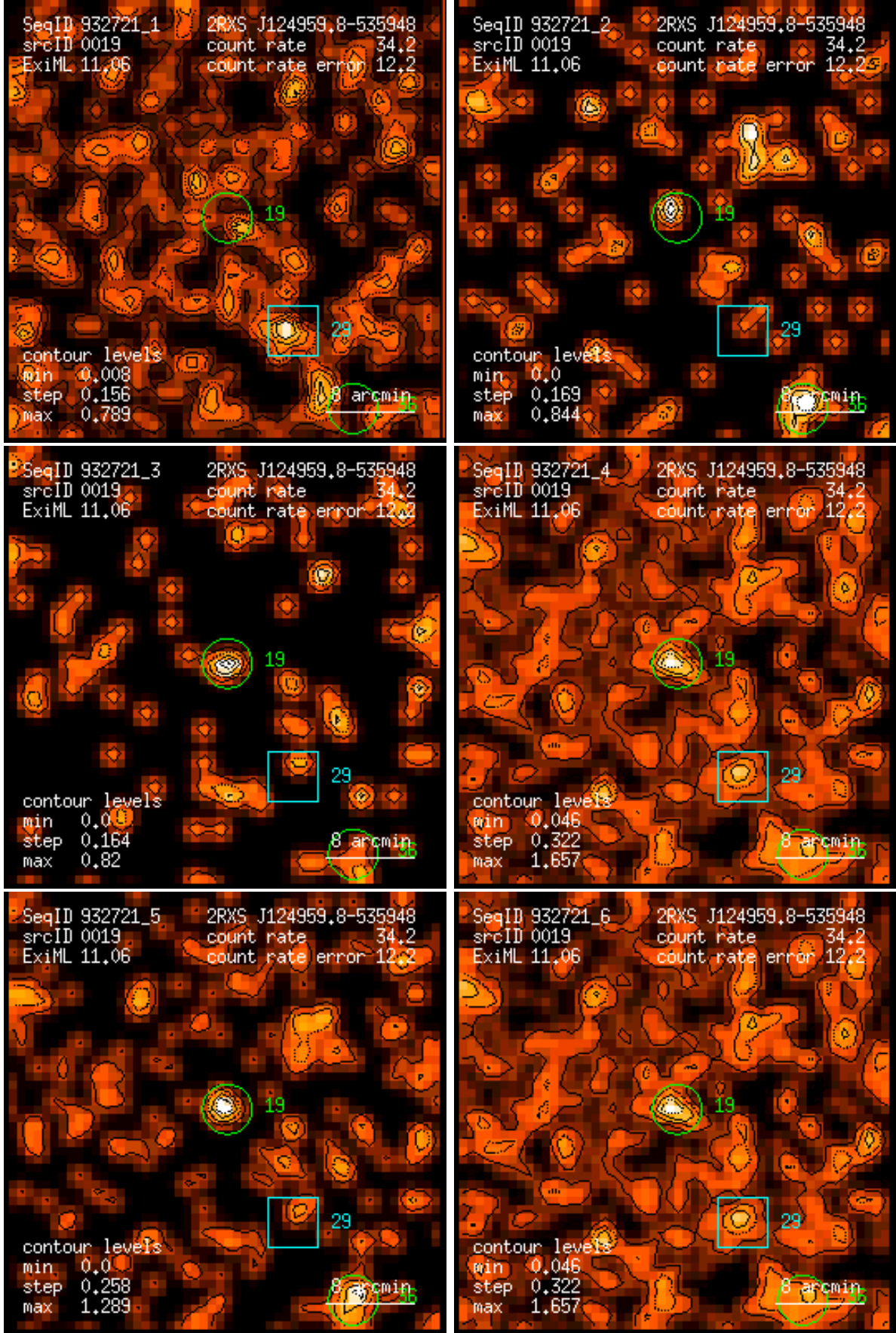
Figure 19: RASS 932721: detection 0019: band rate images, Gaussian filter: (1) PSPC channels 11 – 41, (2) 52 – 90, (3) 91 – 201, (4) 11 – 235, (5) 52 – 201, (6) 11 – 201. Broad band rates in counts/ks. Band rate contour levels in counts/ks/arcmin 2 .
