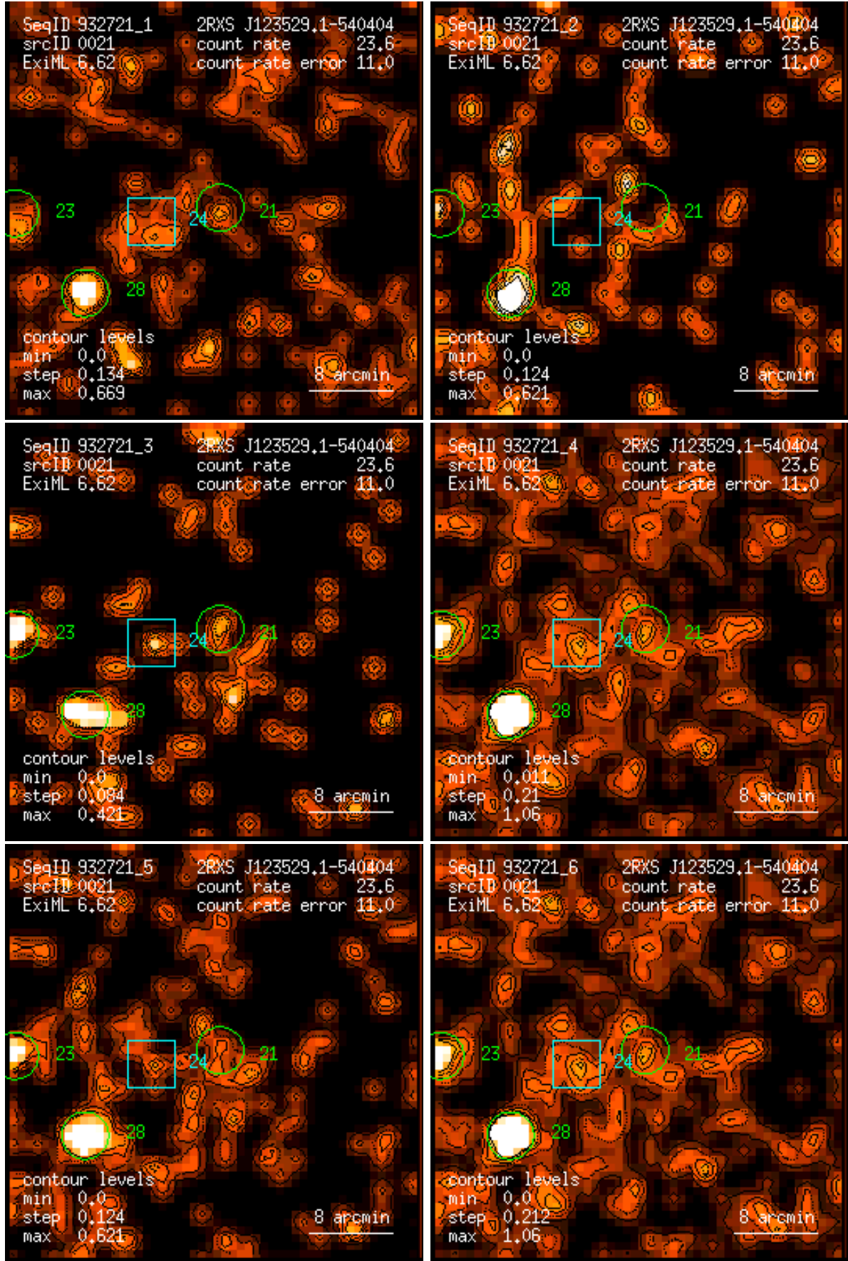
Figure 21: RASS 932721: detection 0021: band rate images, Gaussian filter: (1) PSPC channels 11 – 41, (2) 52 – 90, (3) 91 – 201, (4) 11 – 235, (5) 52 – 201, (6) 11 – 201. Broad band rates in counts/ks. Band rate contour levels in counts/ks/arcmin 2 .
