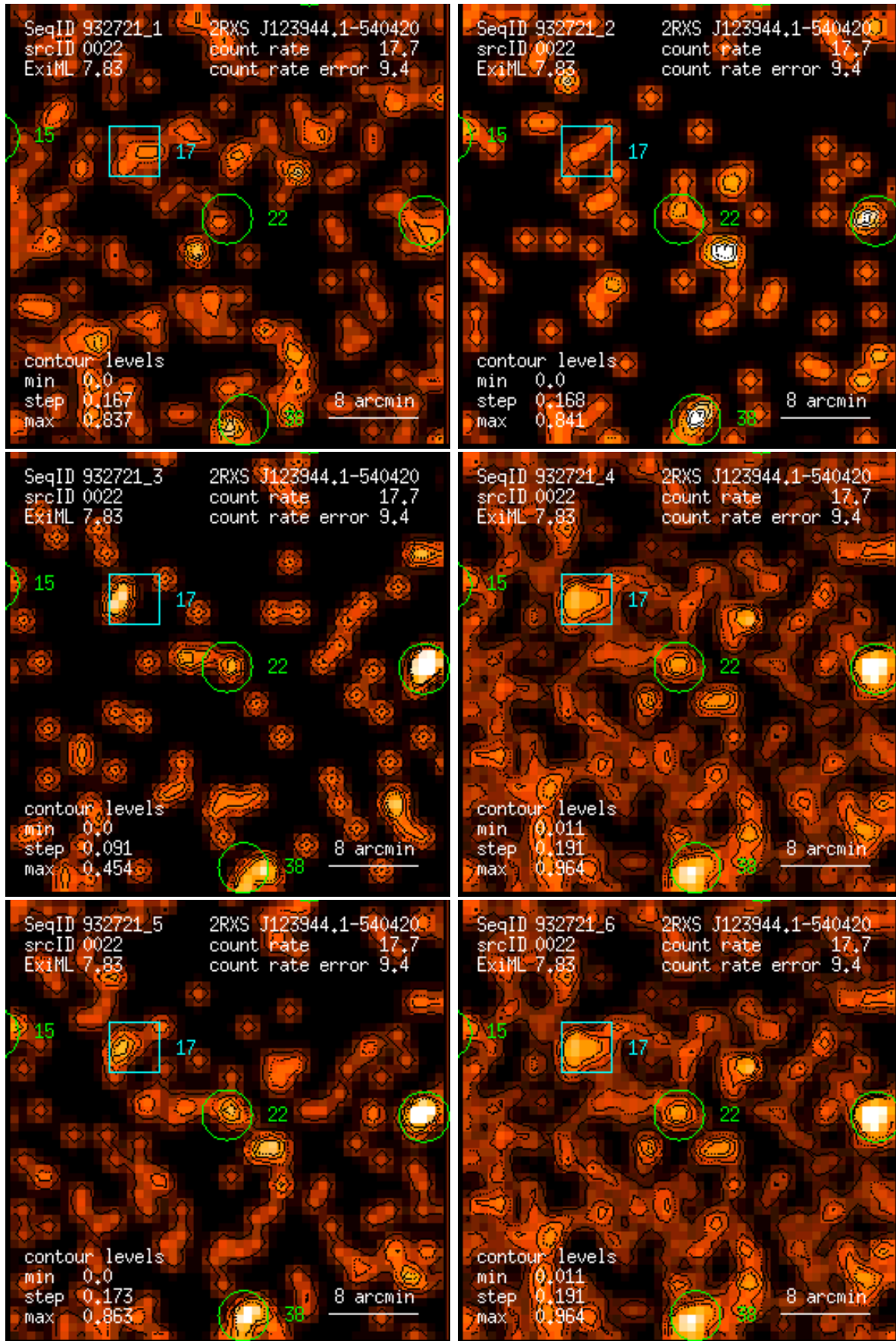
Figure 22: RASS 932721: detection 0022: band rate images, Gaussian filter: (1) PSPC channels 11 – 41, (2) 52 – 90, (3) 91 – 201, (4) 11 – 235, (5) 52 – 201, (6) 11 – 201. Broad band rates in counts/ks. Band rate contour levels in counts/ks/arcmin 2 .
