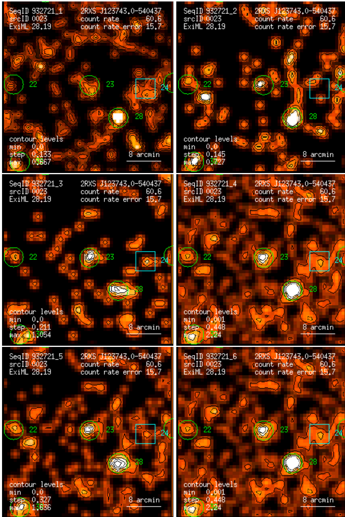
Figure 23: RASS 932721: detection 0023: band rate images, Gaussian filter: (1) PSPC channels 11 – 41, (2) 52 – 90, (3) 91 – 201, (4) 11 – 235, (5) 52 – 201, (6) 11 – 201. Broad band rates in counts/ks. Band rate contour levels in counts/ks/arcmin 2 .
