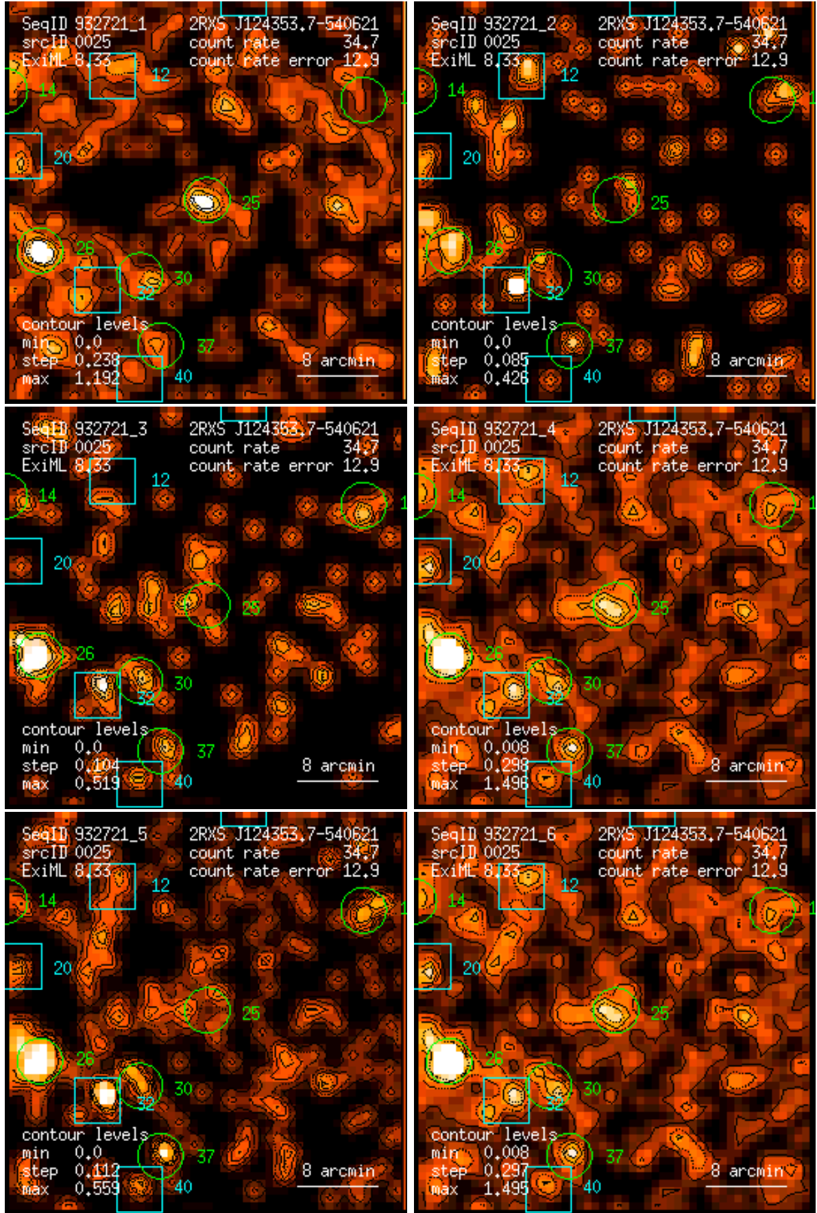
Figure 25: RASS 932721: detection 0025: band rate images, Gaussian filter: (1) PSPC channels 11 – 41, (2) 52 – 90, (3) 91 – 201, (4) 11 – 235, (5) 52 – 201, (6) 11 – 201. Broad band rates in counts/ks. Band rate contour levels in counts/ks/arcmin 2 .
