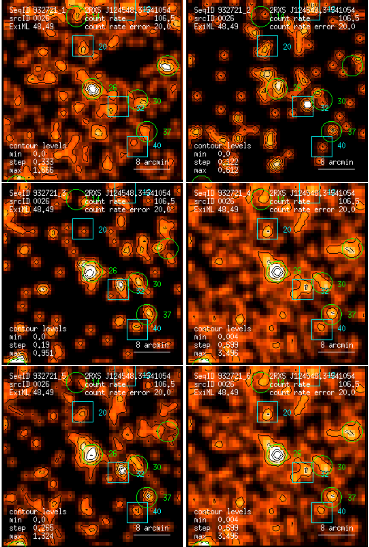
Figure 26: RASS 932721: detection 0026: band rate images, Gaussian filter: (1) PSPC channels 11 – 41, (2) 52 – 90, (3) 91 – 201, (4) 11 – 235, (5) 52 – 201, (6) 11 – 201. Broad band rates in counts/ks. Band rate contour levels in counts/ks/arcmin 2 .
