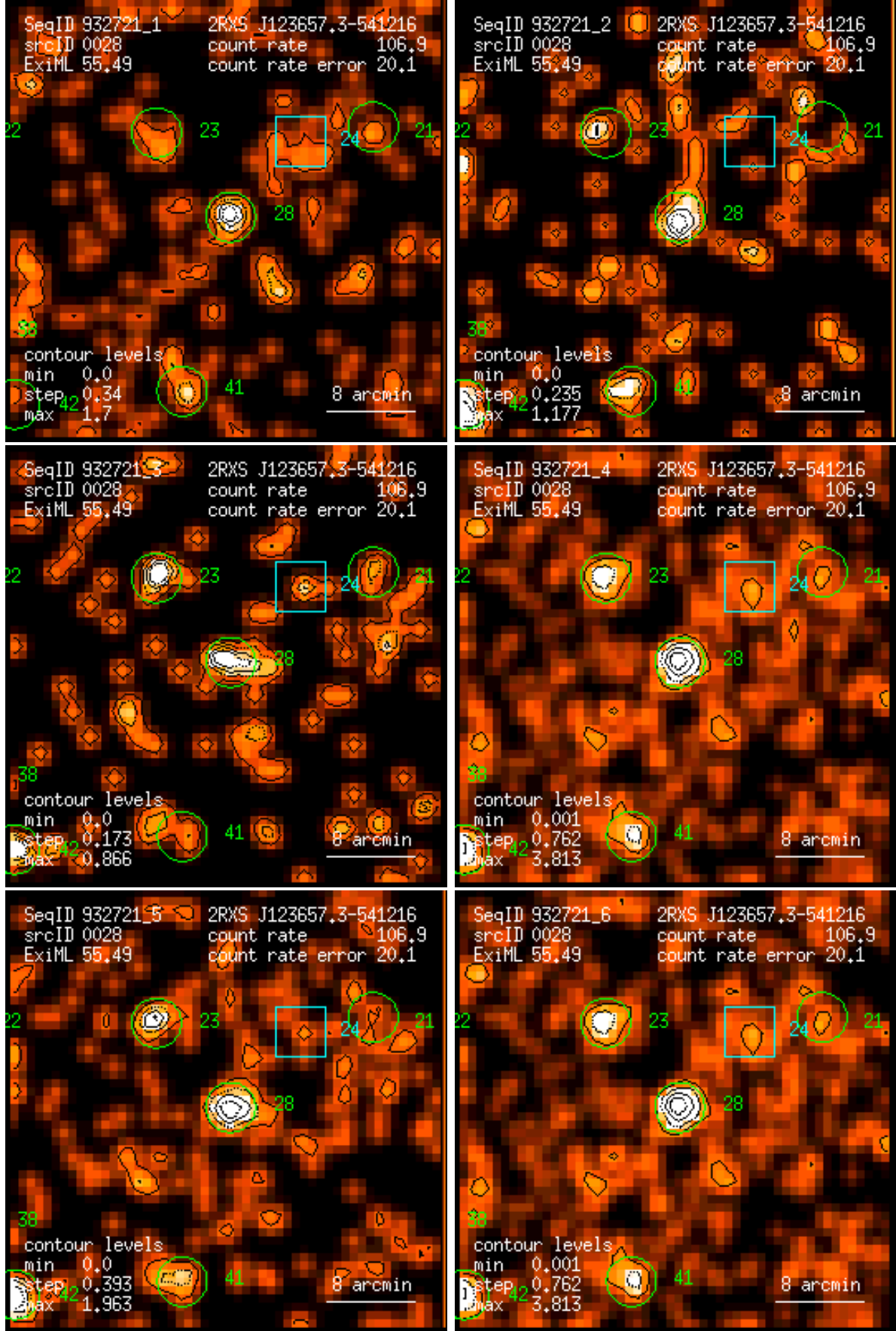
Figure 28: RASS 932721: detection 0028: band rate images, Gaussian filter: (1) PSPC channels 11 – 41, (2) 52 – 90, (3) 91 – 201, (4) 11 – 235, (5) 52 – 201, (6) 11 – 201. Broad band rates in counts/ks. Band rate contour levels in counts/ks/arcmin 2 .
