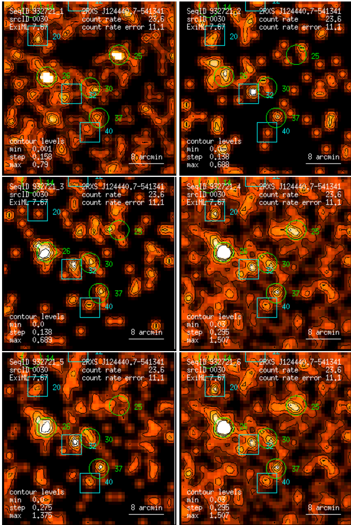
Figure 30: RASS 932721: detection 0030: band rate images, Gaussian filter: (1) PSPC channels 11 – 41, (2) 52 – 90, (3) 91 – 201, (4) 11 – 235, (5) 52 – 201, (6) 11 – 201. Broad band rates in counts/ks. Band rate contour levels in counts/ks/arcmin 2 .
