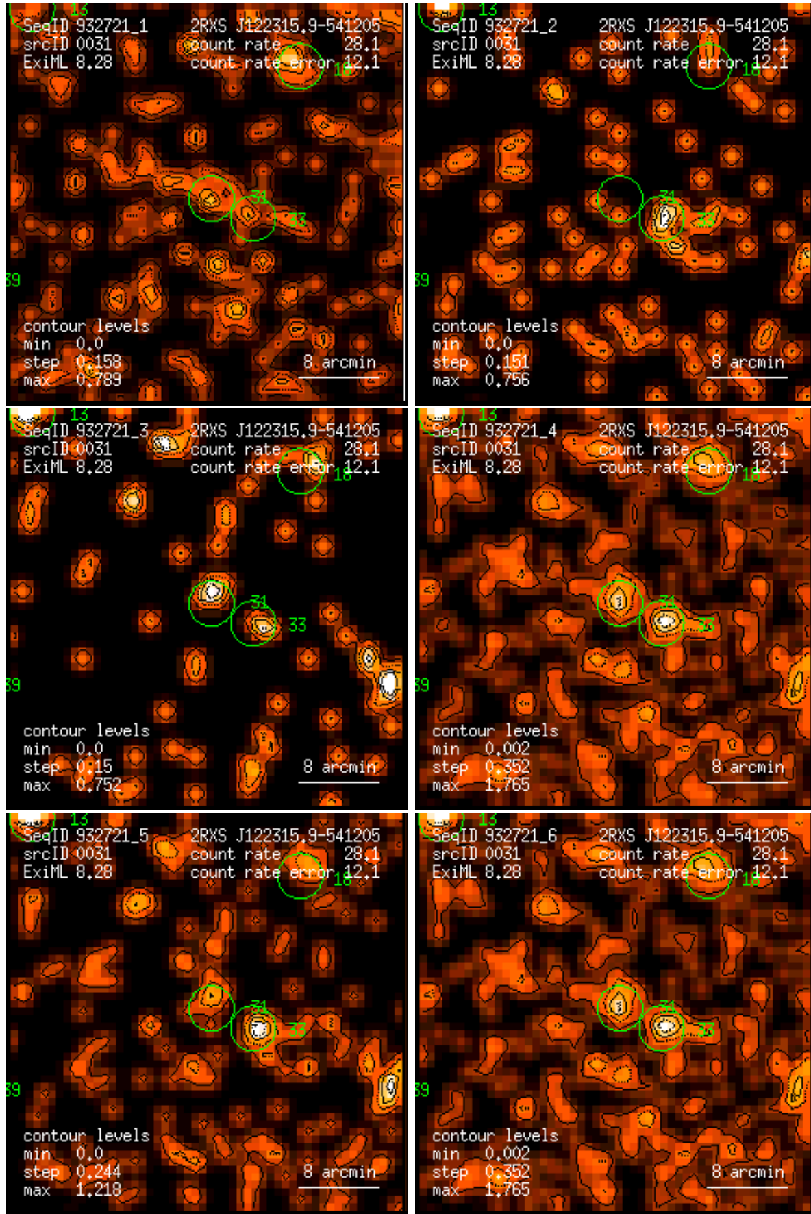
Figure 31: RASS 932721: detection 0031: band rate images, Gaussian filter: (1) PSPC channels 11 – 41, (2) 52 – 90, (3) 91 – 201, (4) 11 – 235, (5) 52 – 201, (6) 11 – 201. Broad band rates in counts/ks. Band rate contour levels in counts/ks/arcmin 2 .
